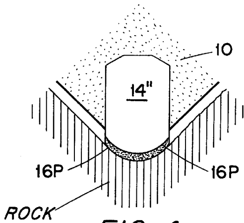
FIG. 4 (PRIOR ART)
