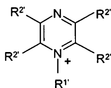
Pyrazinium
