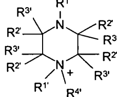
Piperazinium
