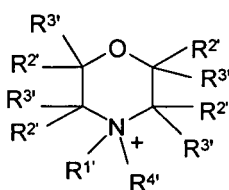
Morpholinium
