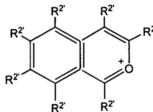
Isochromylium (2-Benzopyrylium)
