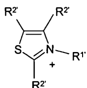
Thiazolium
