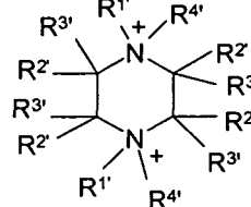
Piperazinium
