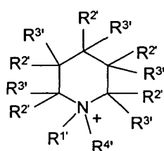
Piperidinium
