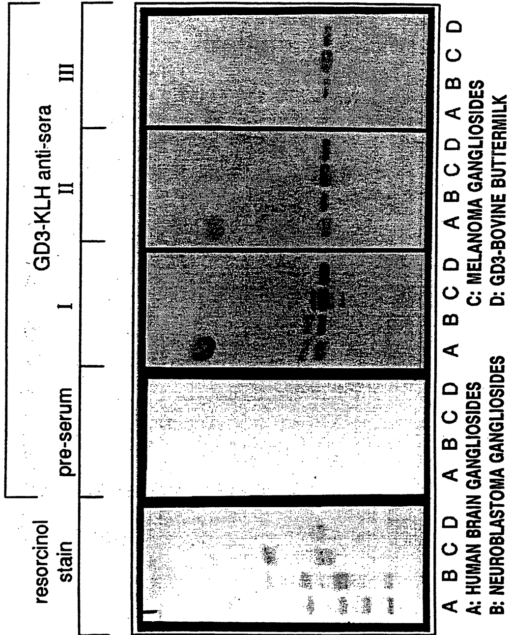
FIGURE 3B IgM
