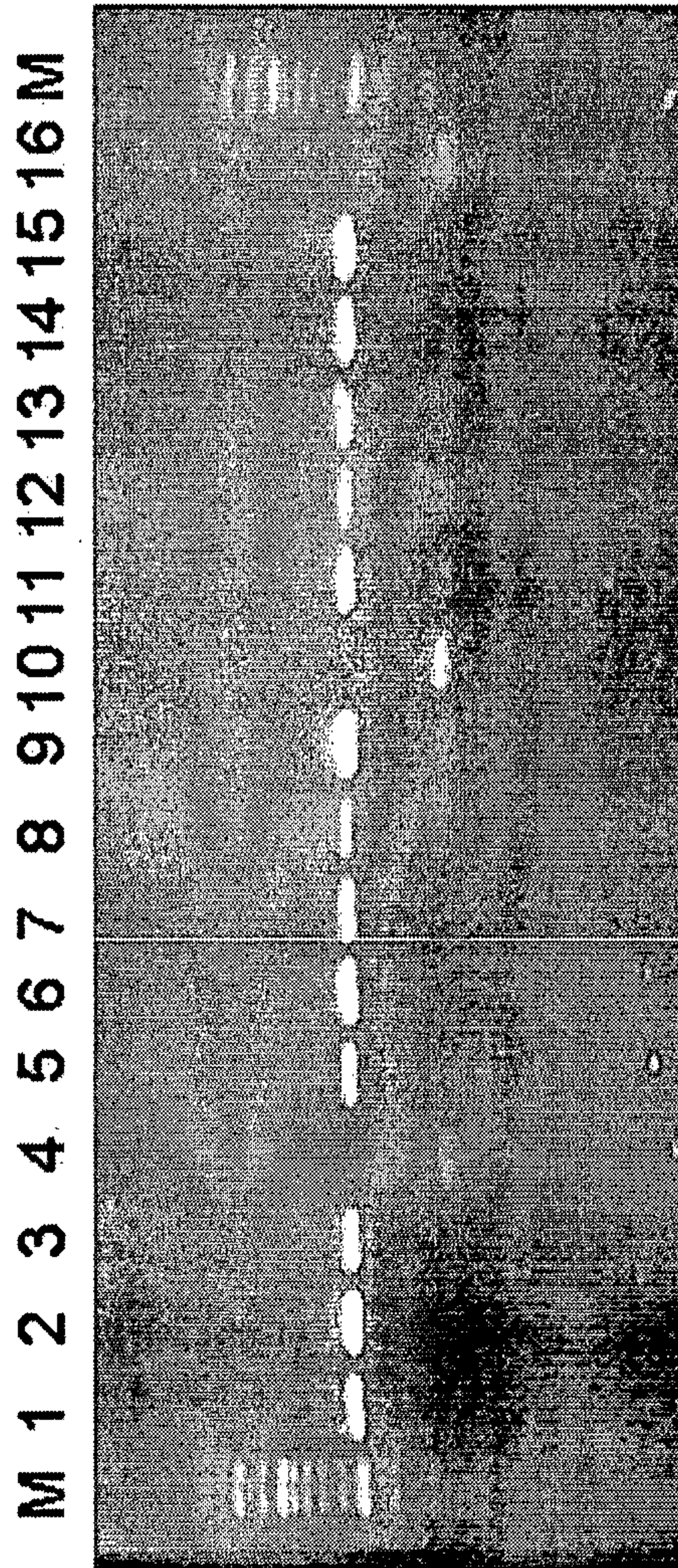
Examples of Genotypes for the CAST SNP:
