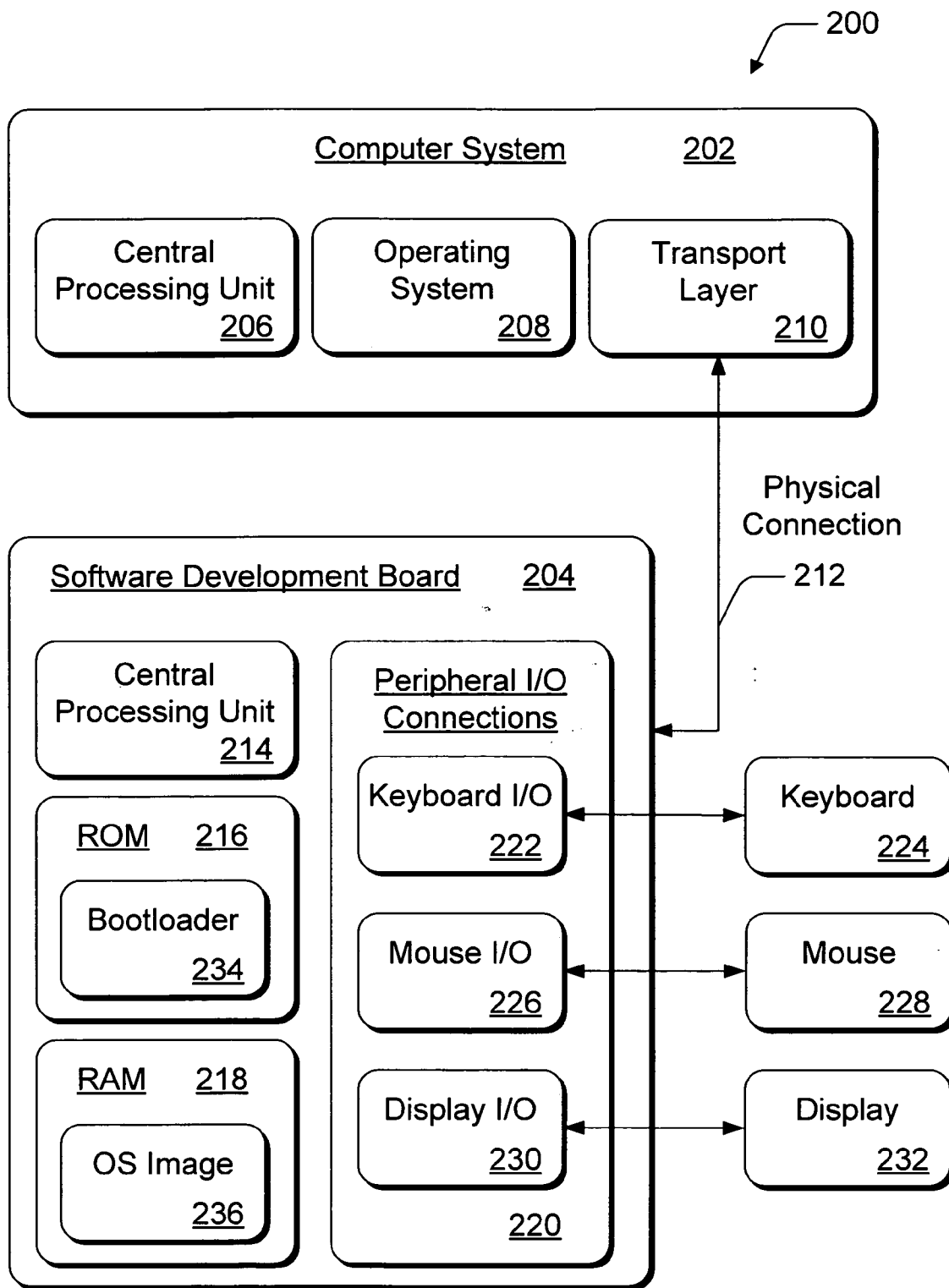
Fig. 2 Prior Art
