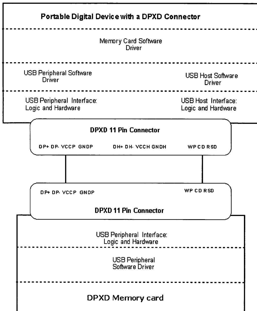
Figure 4: A Portable Digital Device with a DPXD Connector Interfaced to a DPXD Memory Card
