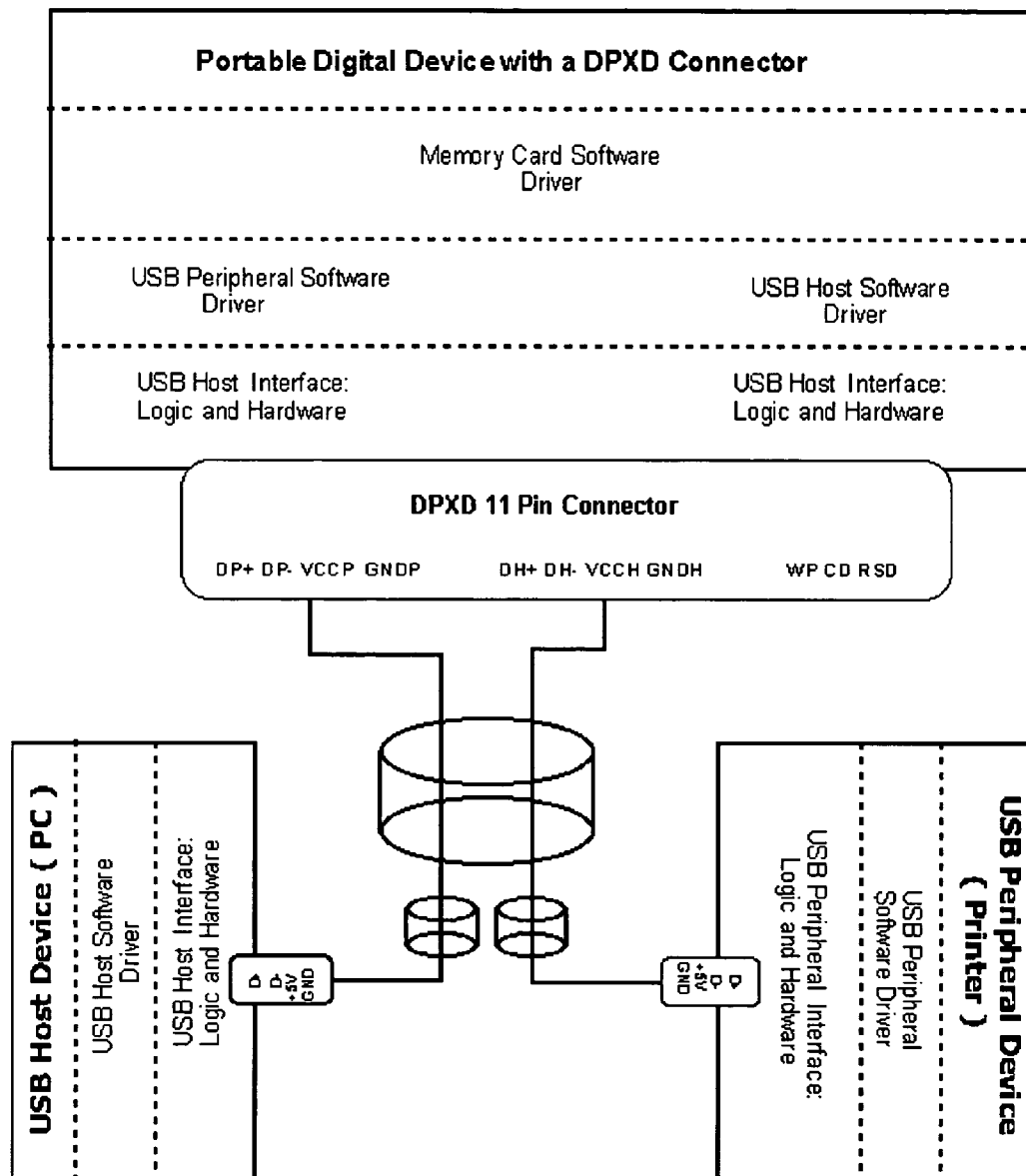
Figure 3: A Portable Digital Device with a DPXD Connector Interfaced to a USB Host Device and a USB Peripheral Device
