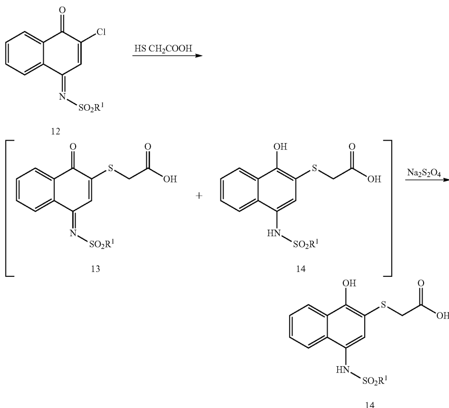
Scheme 7: in situ reduction of naphthoquinone sulfonimide derivatives 13 to the final hydronaphthoquinone sulfonamide derivatives 14
