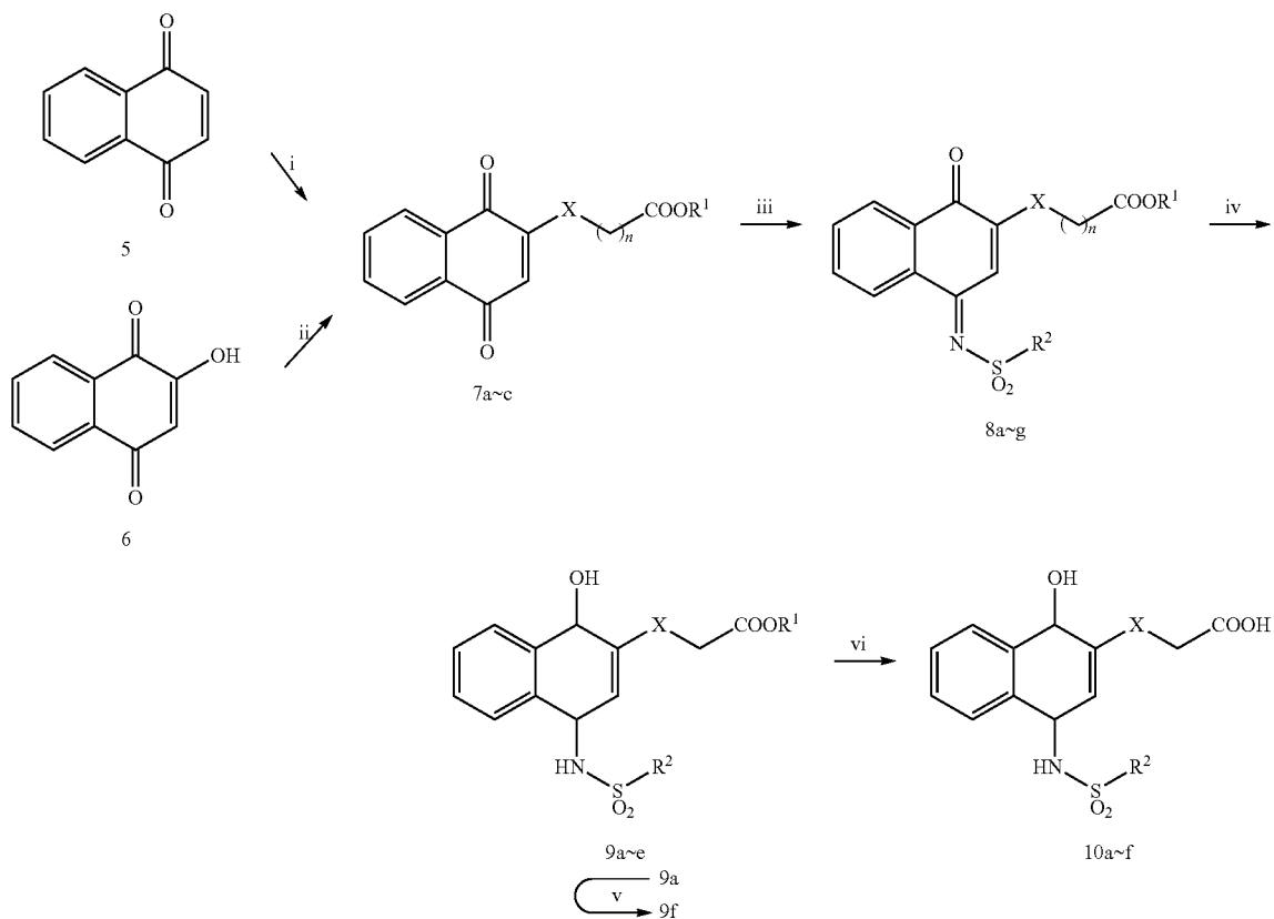
Scheme 5,
