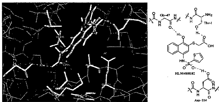
Figure 13: H-bonding interaction between HLM-008182 and chymotrypsin-like catalytic site of 20S proteasome predicted by molecular modeling.
