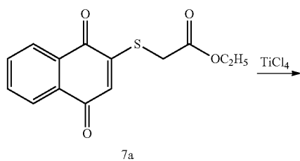
Scheme 8: proposed mechanism for regioselective coupling of sulfonamide to 1,4-naphthoquinone derivative using compound 7a as an example.
