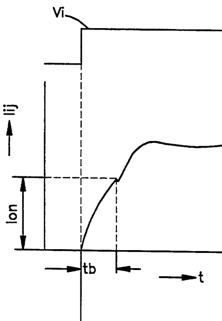
FIG.6 (PRIOR ART)
