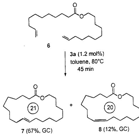
Scheme 2. Stereochemistry
