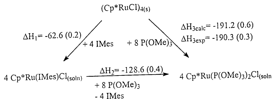
Scheme 1. Thermodynamic Cycle
