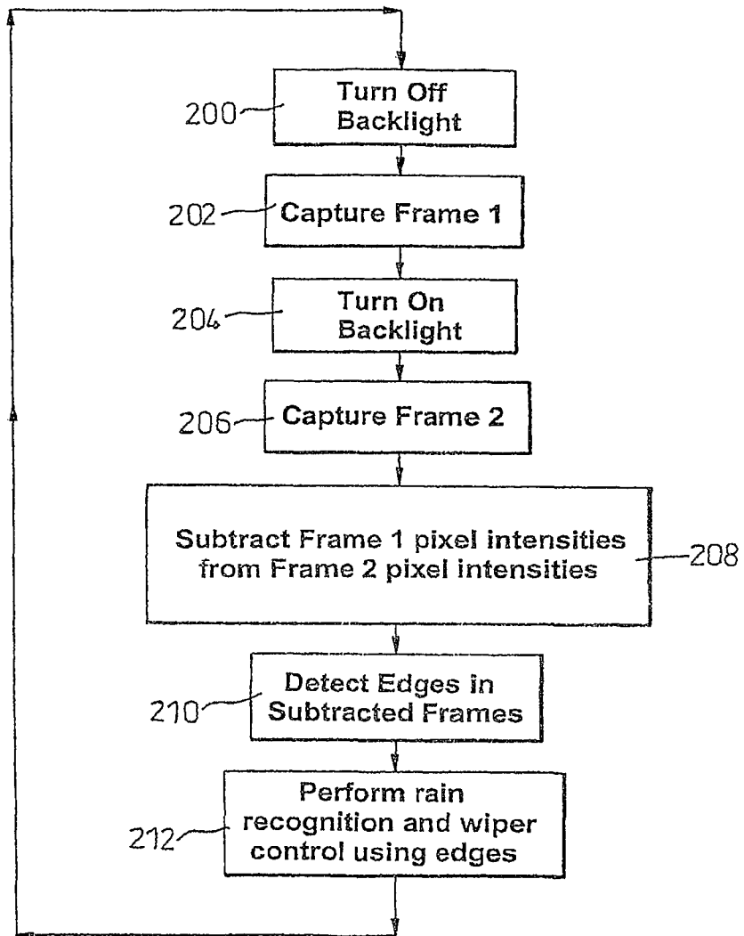
Frame Subtraction Control Diagram
