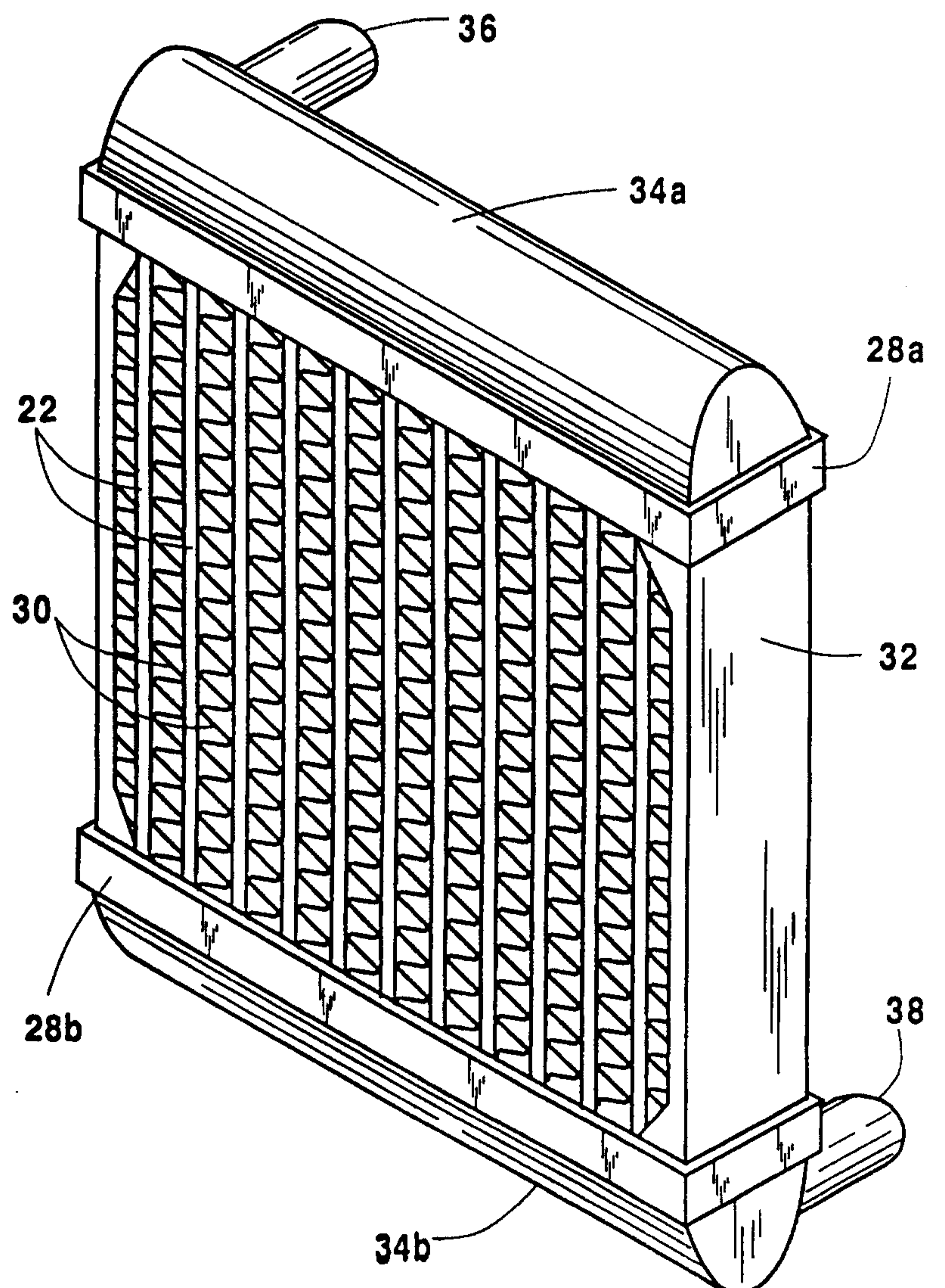
Fig. 2 (PRIOR ART)
