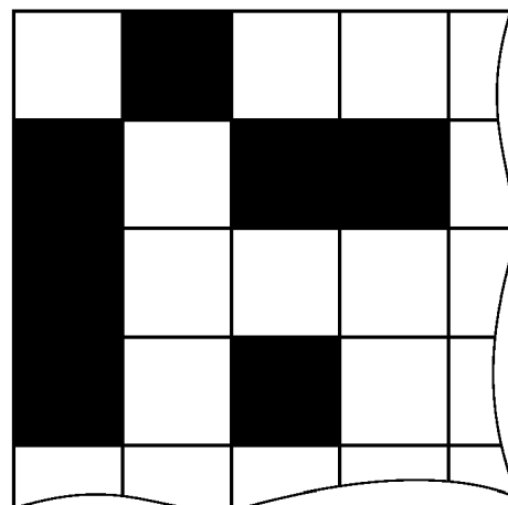
FOURTH SCANNING
