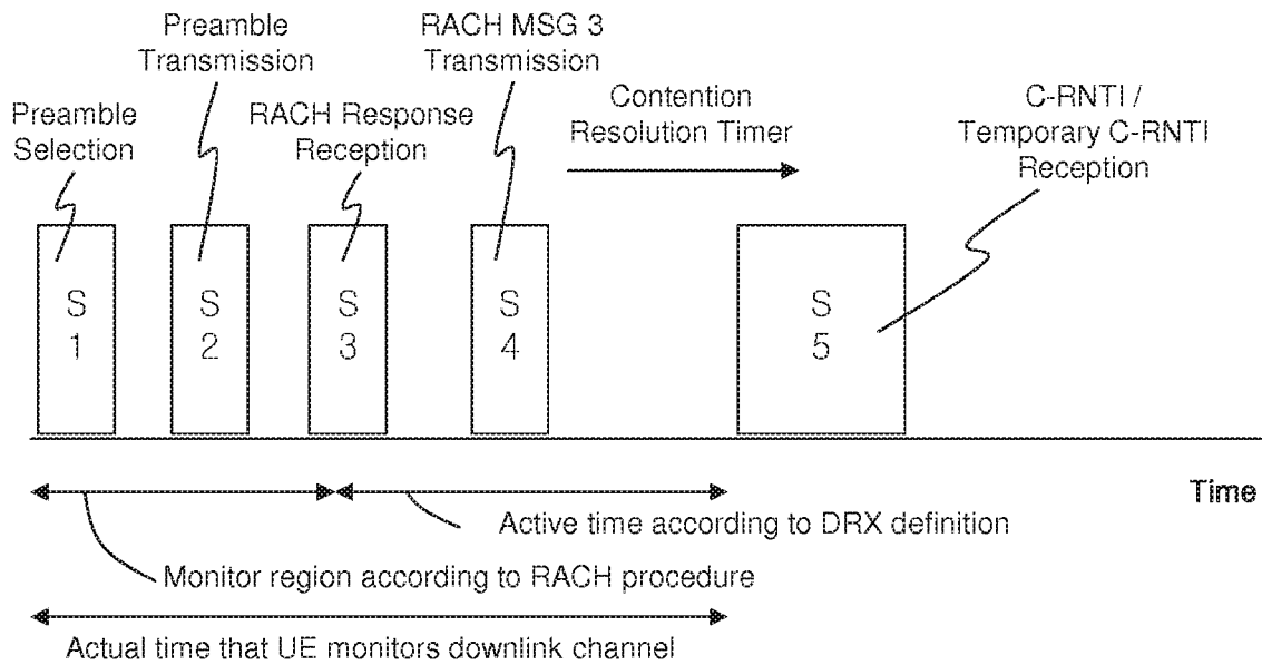
(a) Contention based RACH
