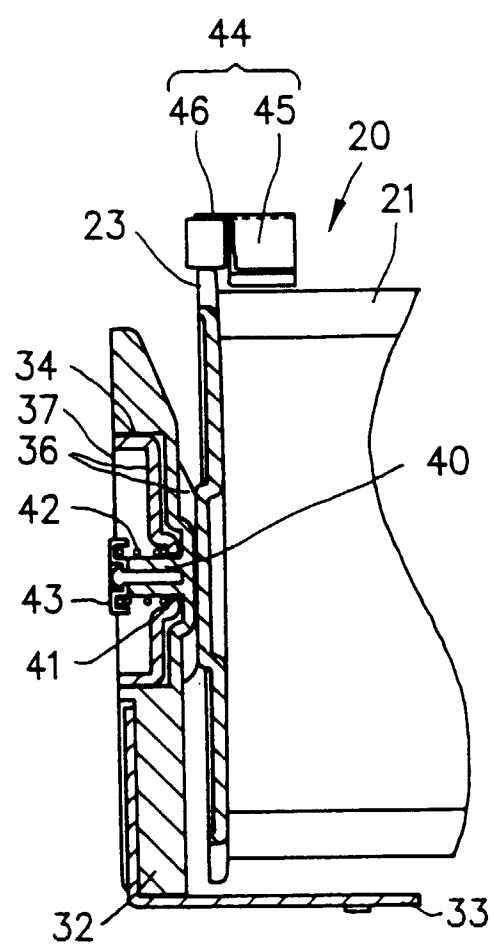
SECTION 3-3
