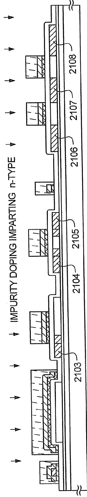
FIG. 21B FORMING n-- REGION
