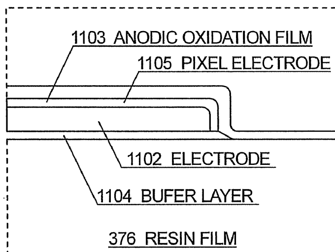
SCHEMATIC DIAGRAM OF ENLARGED ELECTRODE EDGE PORTION
