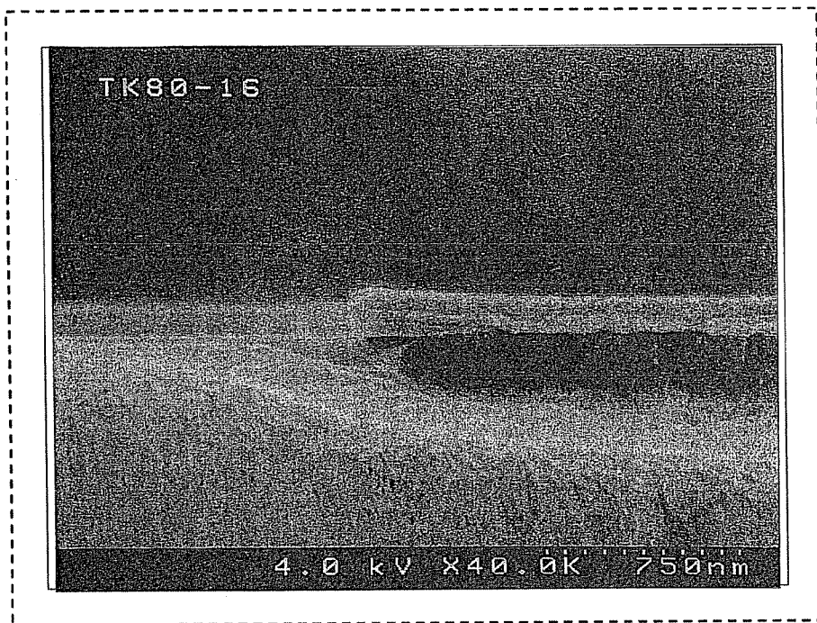
SEM PHOTOGRAPH (CROSS SECTION)
