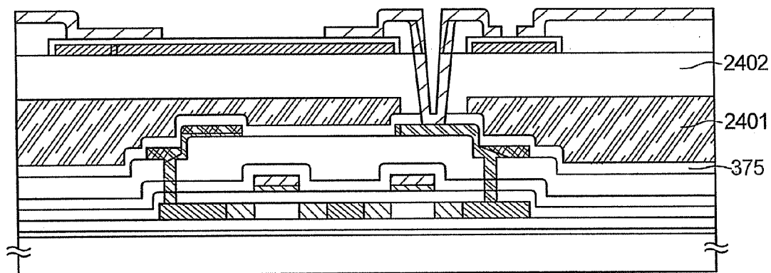
701: n-CHANNEL TFT
