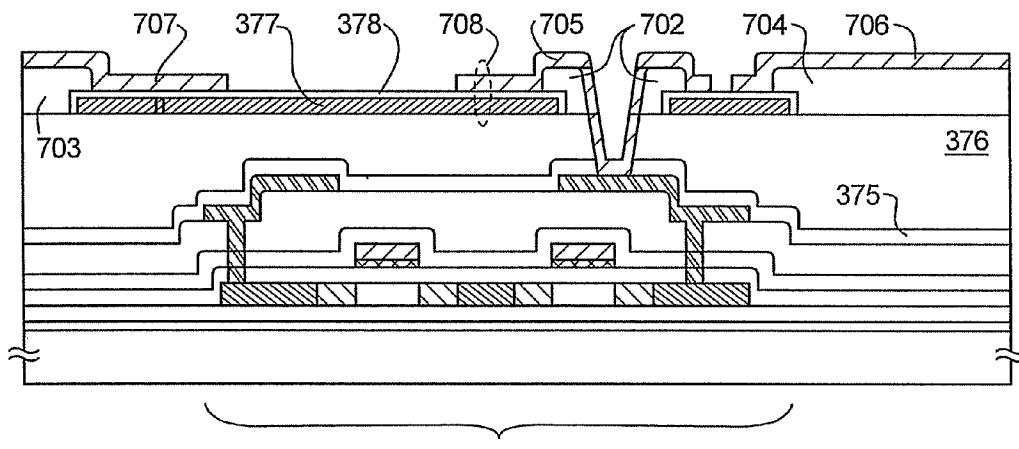
701: n-CHANNEL TFT
