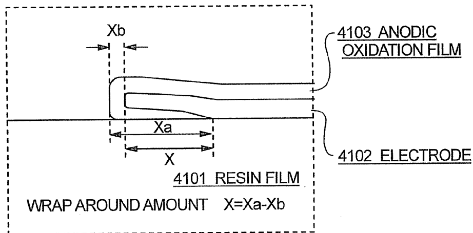
SCHEMATIC DIAGRAM OF ENLARGED ELECTRODE EDGE PORTION
