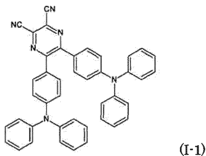
[Chemical formula 35]
