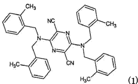
[Chemical formula 1]
