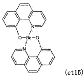
[Chemical formula 185]
