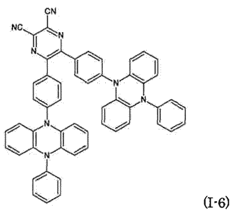
[Chemical formula 40]
