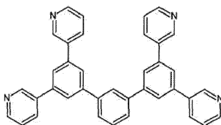
[Chemical formula 220]
