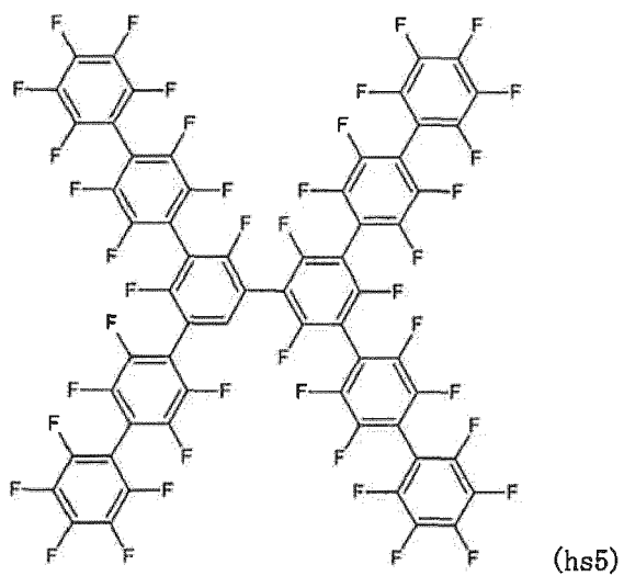
[Chemical formula 164]
