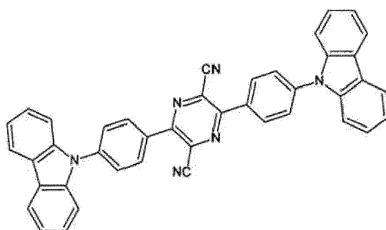
[Chemical formula 49]
