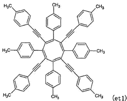
[Chemical formula 171]
