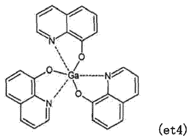
[Chemical formula 174]
