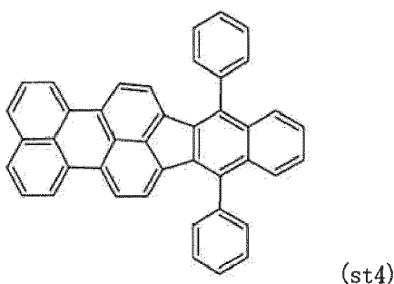
[Chemical formula 208]
