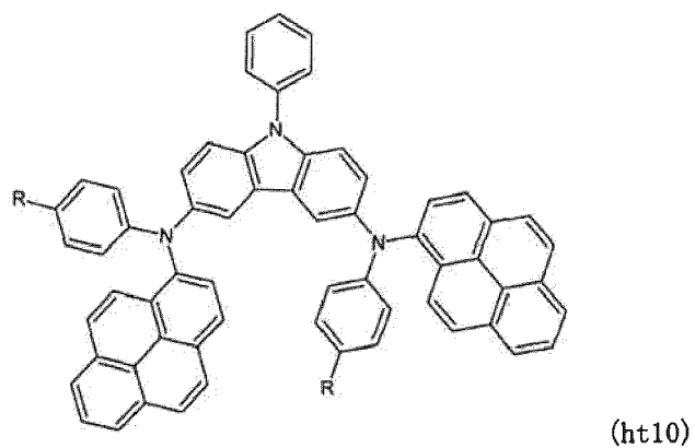
[Chemical formula 86]
