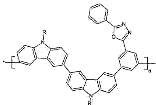
[Chemical formula 156]
