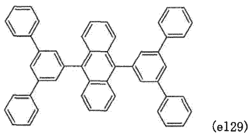
[Chemical formula 148]
