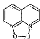
[Chemical formula 200]
