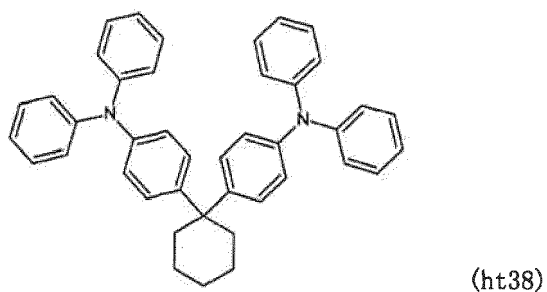
[Chemical formula 113]
