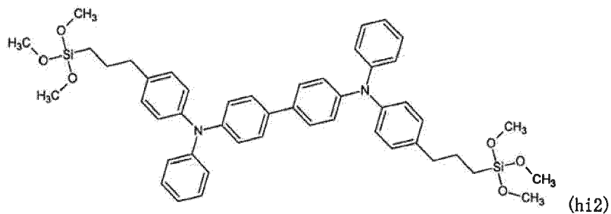
[Chemical formula 71]
