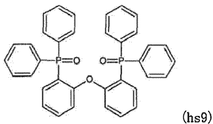
[Chemical formula 168]
