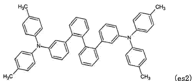
[Chemical formula 116]
