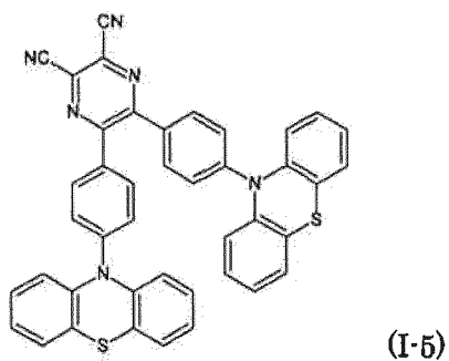
[Chemical formula 39]
