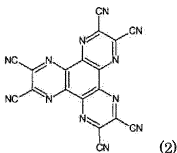
[Chemical formula 3]
