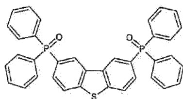
[Chemical formula 199]
