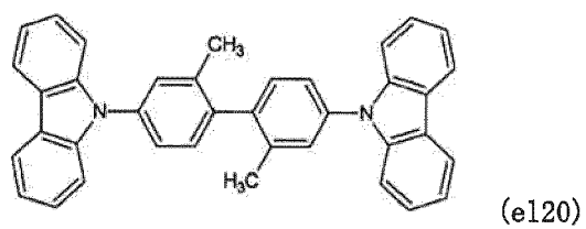
[Chemical formula 138]
