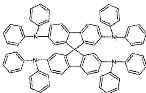
[Chemical formula 122]
