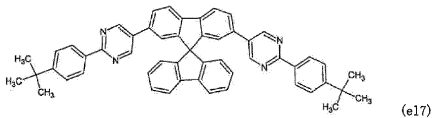
[Chemical formula 126]
