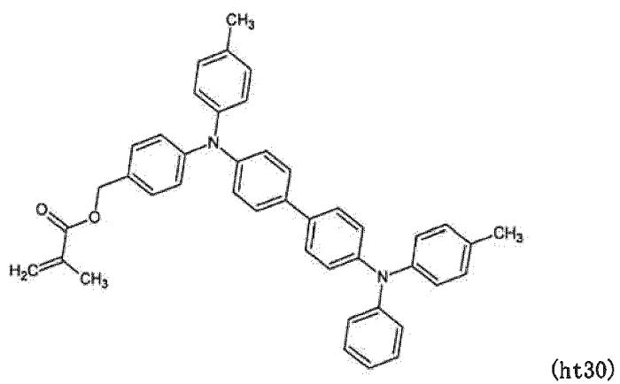
[Chemical formula 106]
