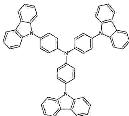
[Chemical formula 91]
