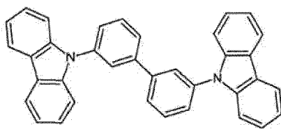
[Chemical formula 211]
