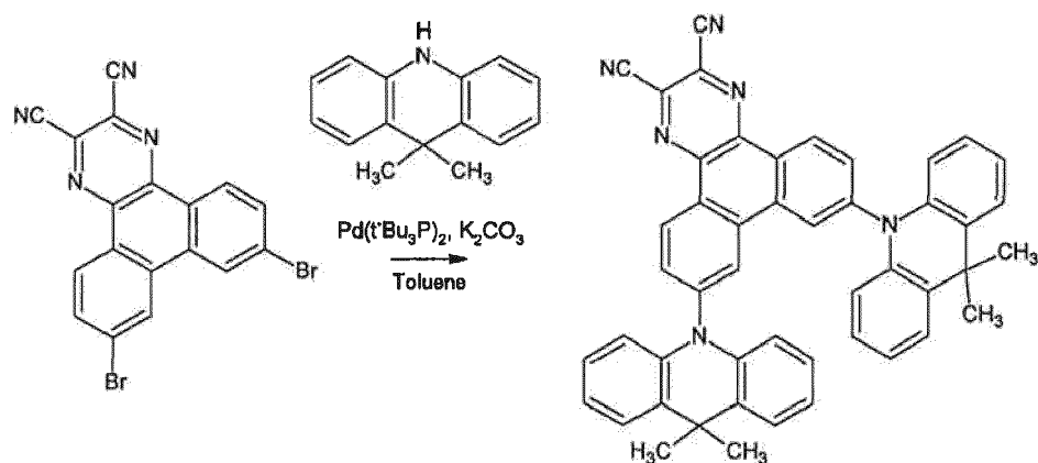
[Chemical formula 63]
