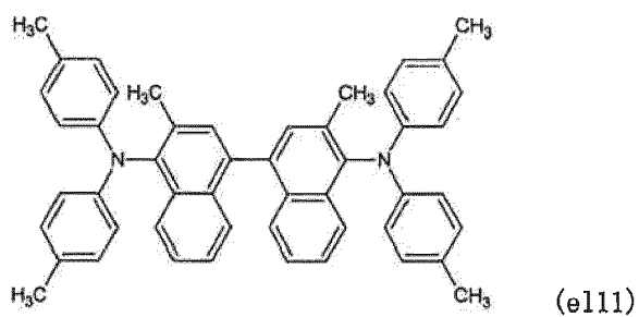
[Chemical formula 130]
