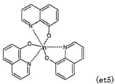
[Chemical formula 175]
