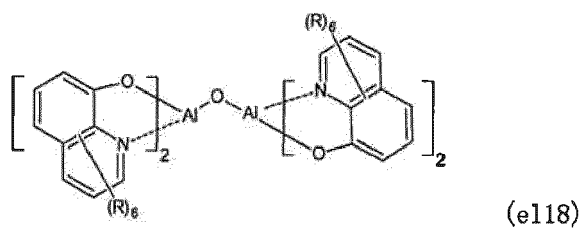
[Chemical formula 137]
