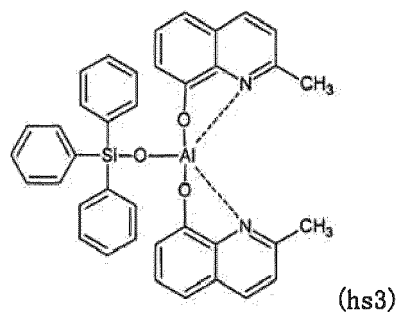
[Chemical formula 162]
