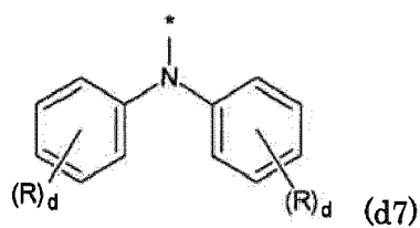
[Chemical formula 21]
