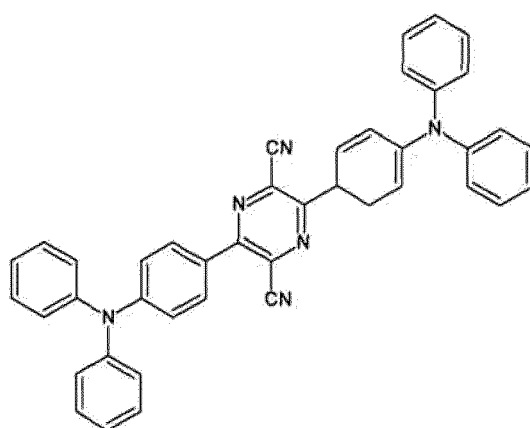
[Chemical formula 48]
