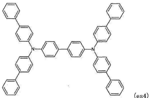
[Chemical formula 118]
