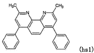
[Chemical formula 160]
