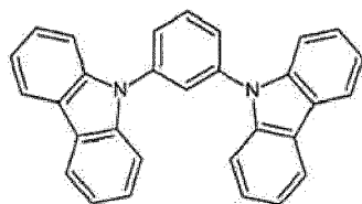
[Chemical formula 210]
