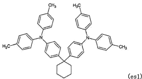
[Chemical formula 115]
