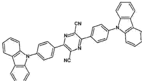
[Chemical formula 219]
