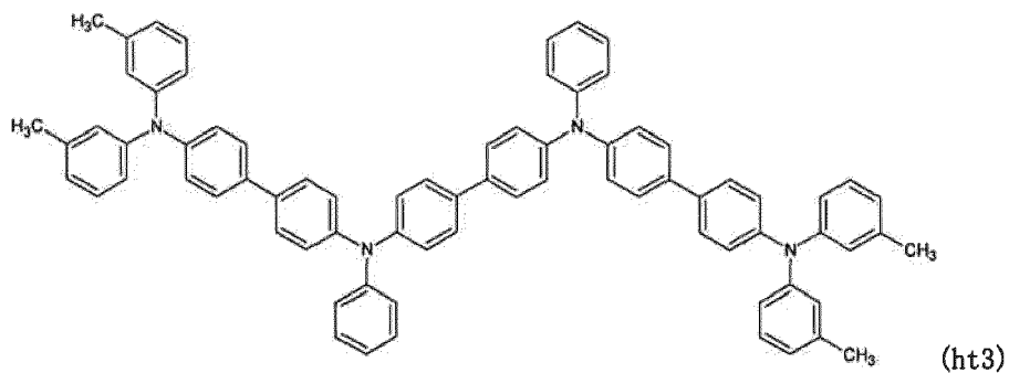
[Chemical formula 78]
