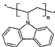
[Chemical formula 155]
