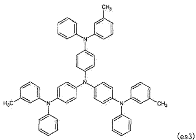
[Chemical formula 116]
