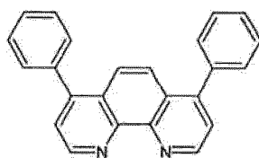
[Chemical formula 199]
