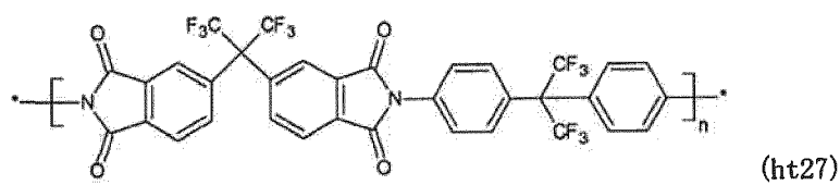
[Chemical formula 103]
