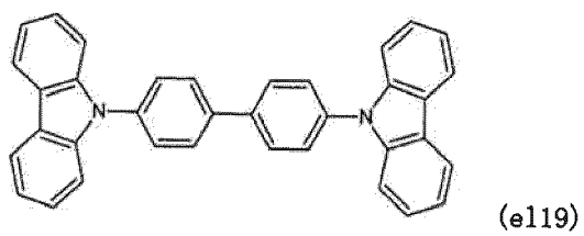
[Chemical formula 138]
