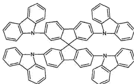
[Chemical formula 122]
