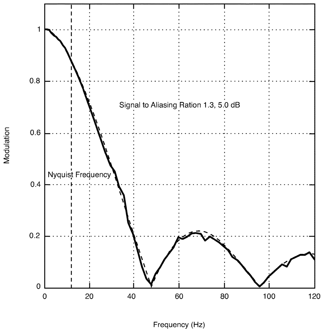
Temporal Modulation Transfer Functions (24 fps, 180 Degree Shutter)
