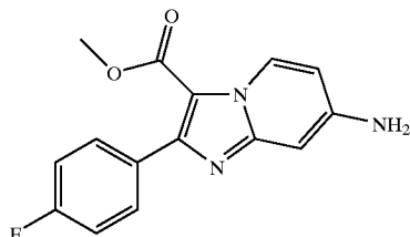
COMPOUND VIIIa:
