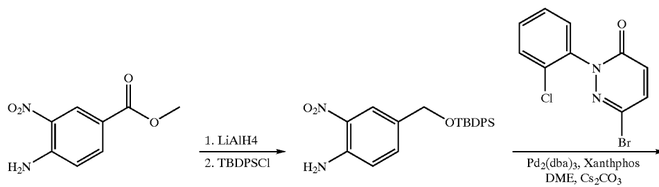
Scheme 5
