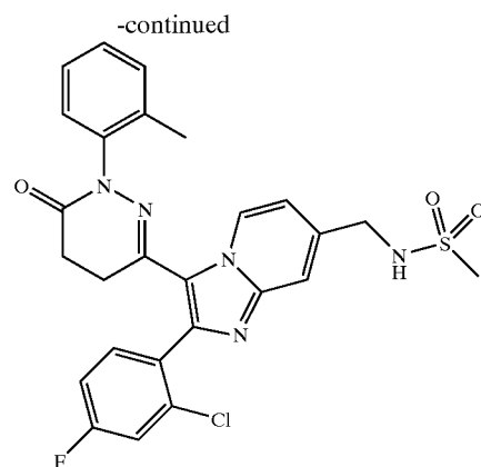
Scheme 3
