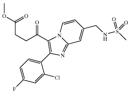
COMPOUND VIa:
