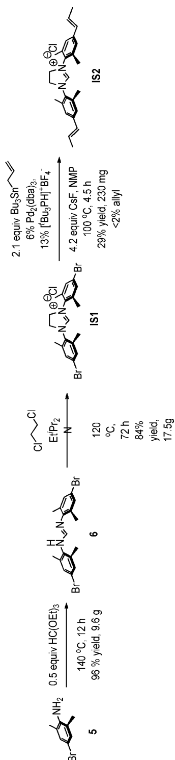
Scheme 1. Synthesis of novel imidazolium salts IS1 and IS2 .
