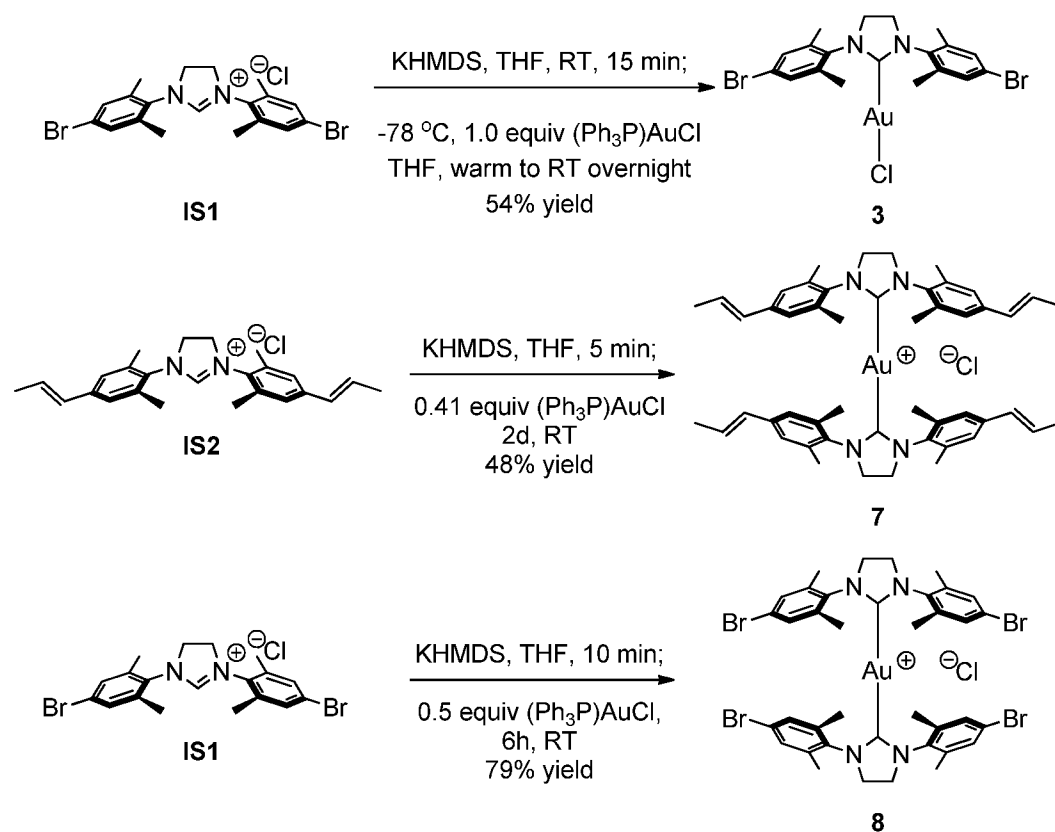
Scheme 2. Synthesis of NHC-Au(I) complexes 3 , 7 , and 8 .
