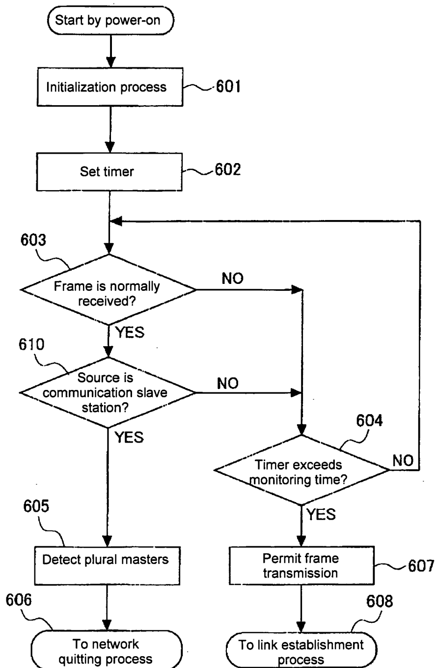
Flowchart showing process performed in communication master station in advance of link establishment process (3)
