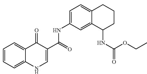
482; [7-[(4-Oxo-1H-quinolin-3-yl)carbonylamino]tetralin-1-yl]aminoformic acid ethyl ester
