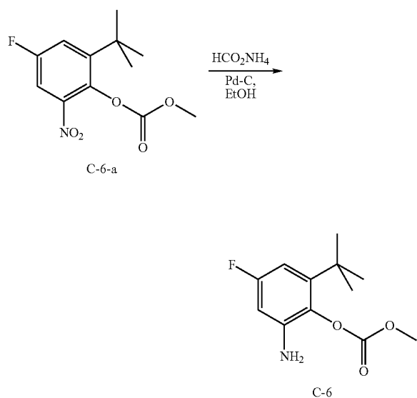
C-6; 2-tert-Butyl-4-fluoro-6-aminophenyl methyl carbonate
