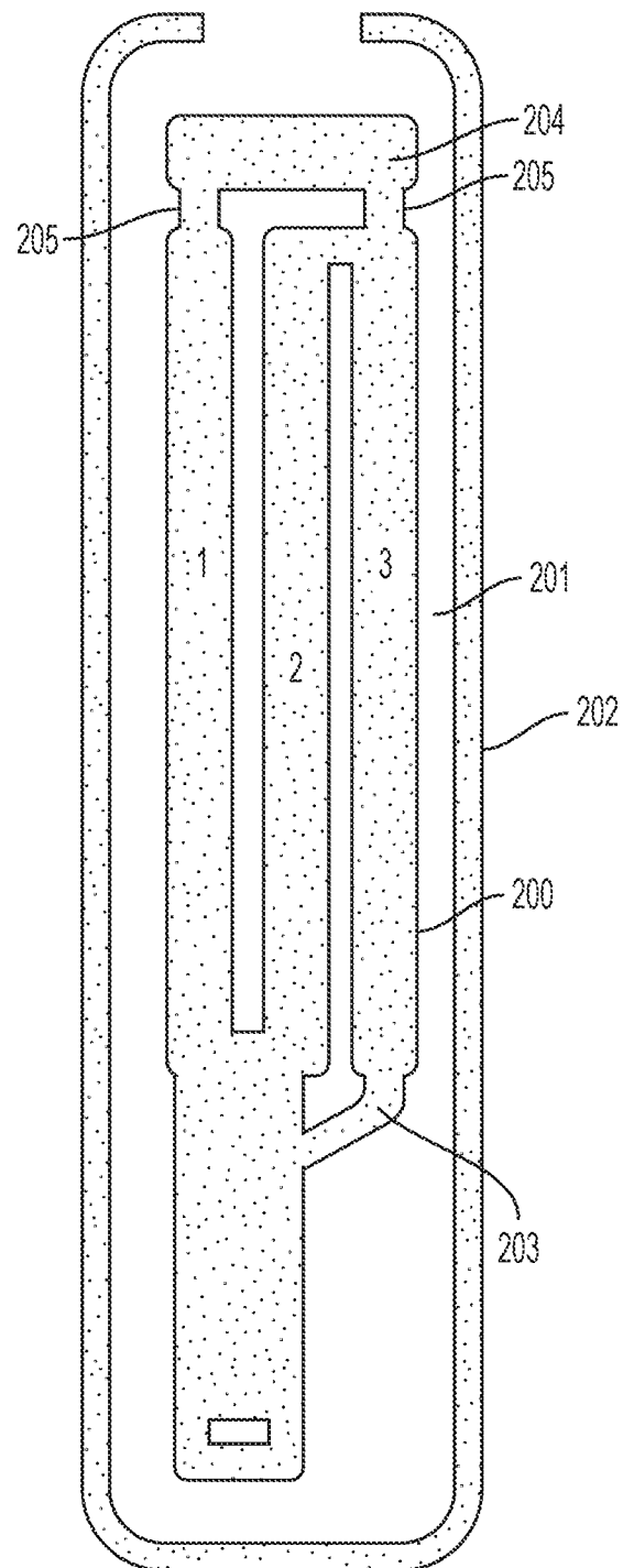
FIG. 2 PRIOR ART
