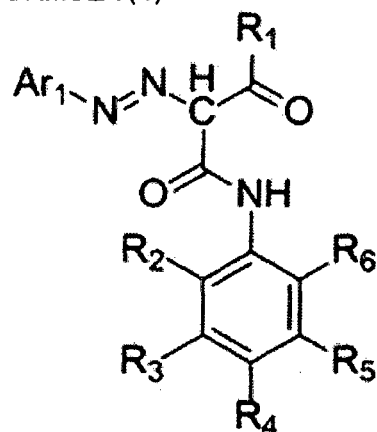
FORMULA (4)
