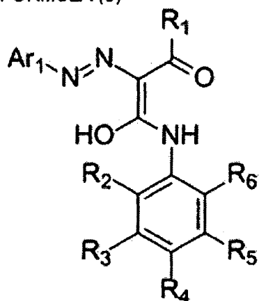
FORMULA (5)
