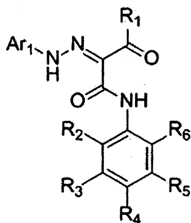
FORMULA (1)
