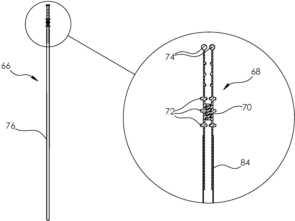
SECTION G-G
