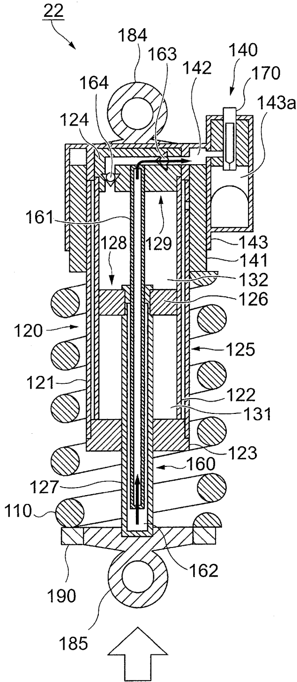
COMPRESSION PROCESS
