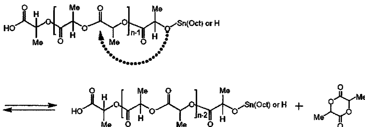
[Reaction Scheme 3]
