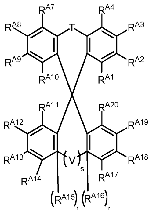
Formula IIc.
