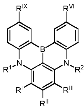
Formula Ie
