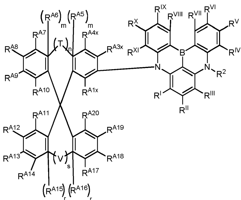
Formula IV
