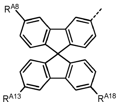
Formula IIj-5
