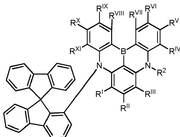
Formula Vb
