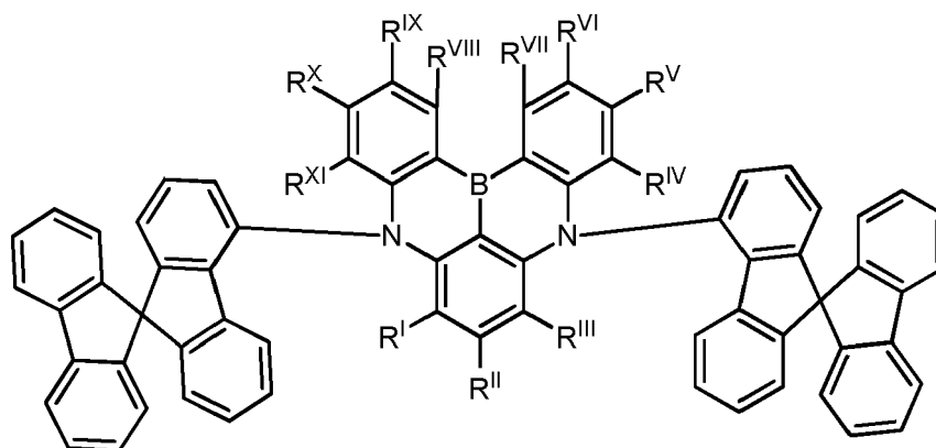
Formula VI-1b
