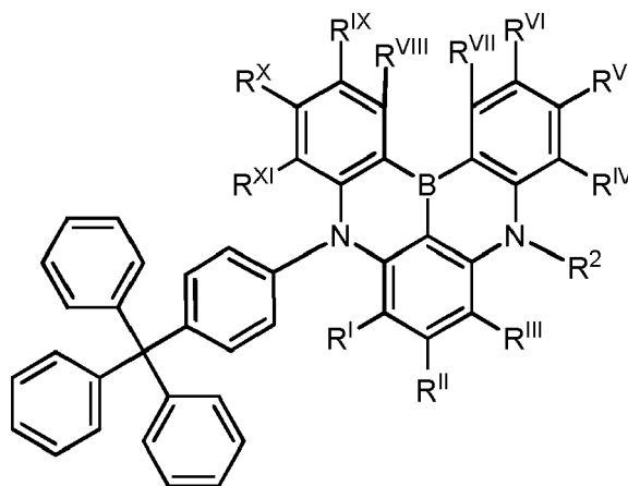
Formula IIIa
