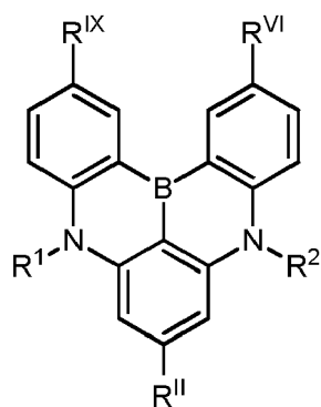
Formula If
