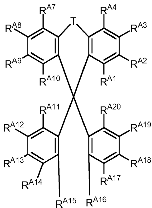
Formula IIh.
