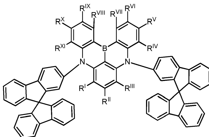
Formula IV-1b
