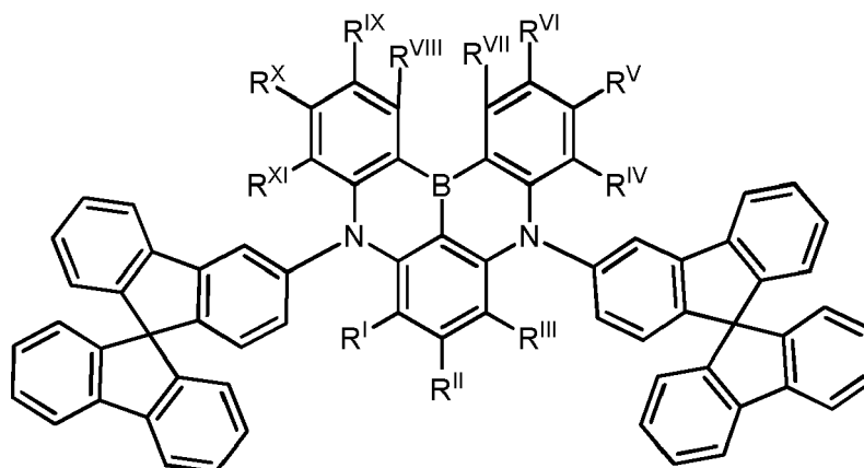
Formula III-1b
