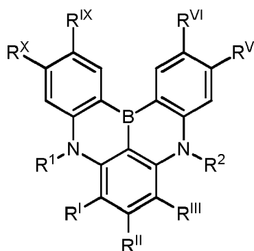
Formula Ia
