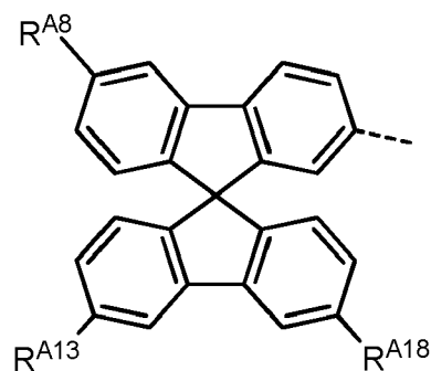
Formula IIj-6
