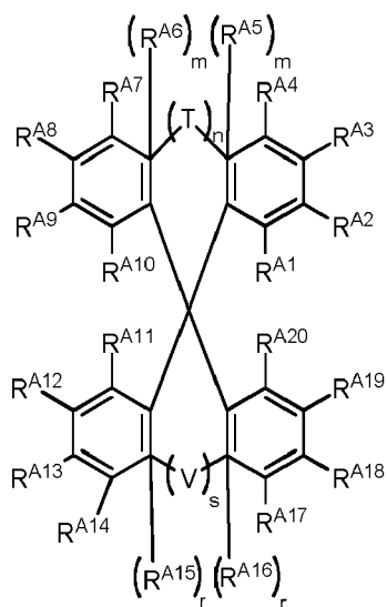
Formula II
