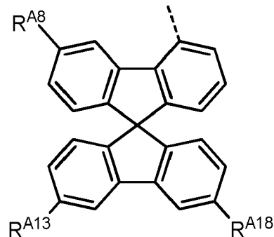
Formula IIj-8
