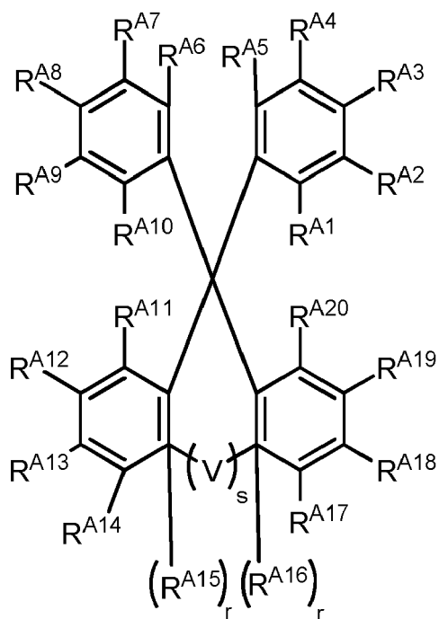
Formula IIa.
