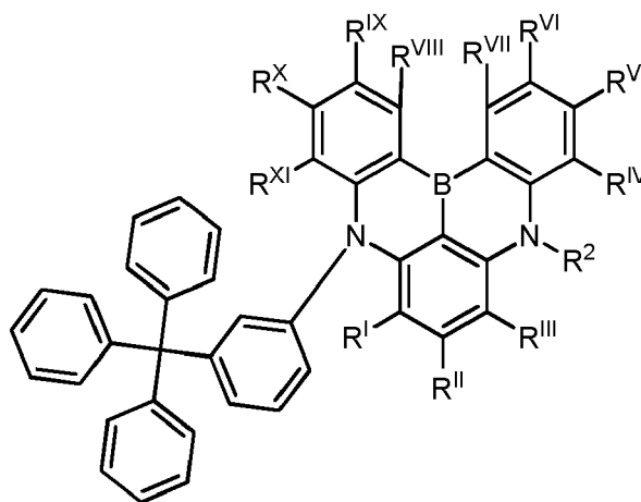
Formula IVa
