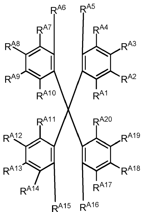
Formula IIe.
