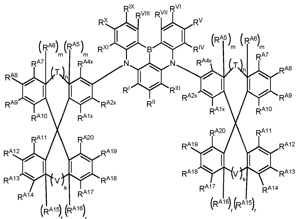
Formula III-1
