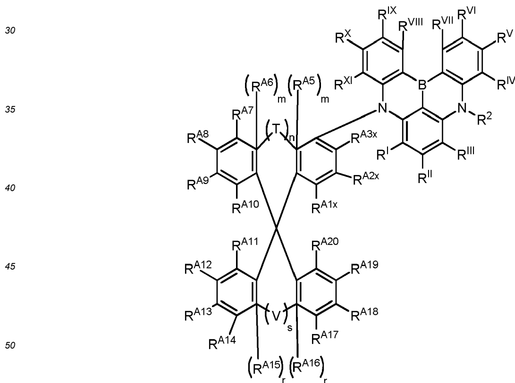
Formula VI
