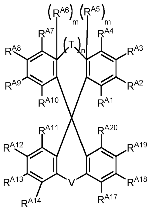
Formula IIc.
