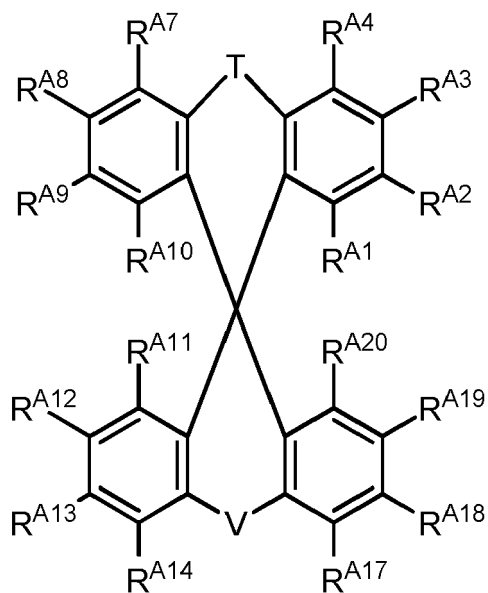
Formula IIf.
