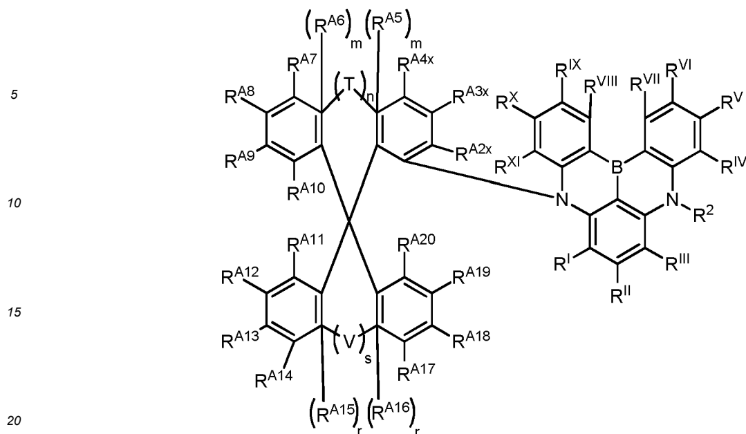
Formula V
