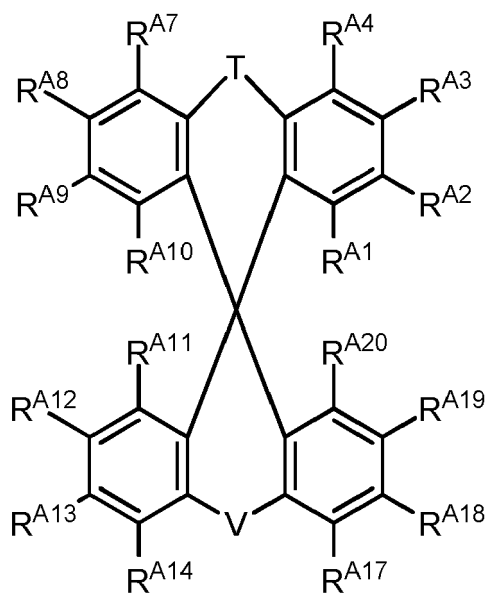
Formula IIe
