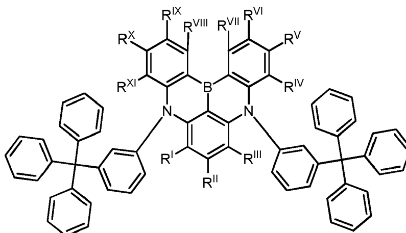
Formula IV-1a
