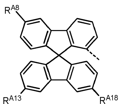
Formula IIj-7
