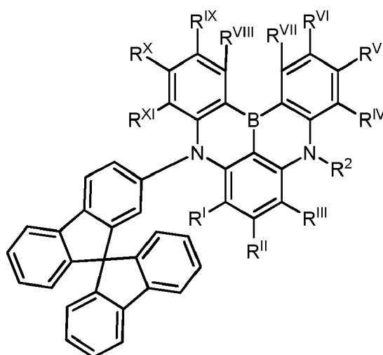
Formula IVb
