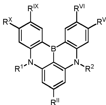
Formula Ib
