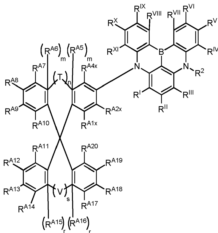
Formula III
