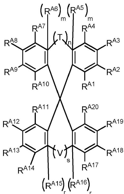
Formula II
