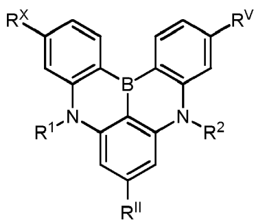
Formula Id
