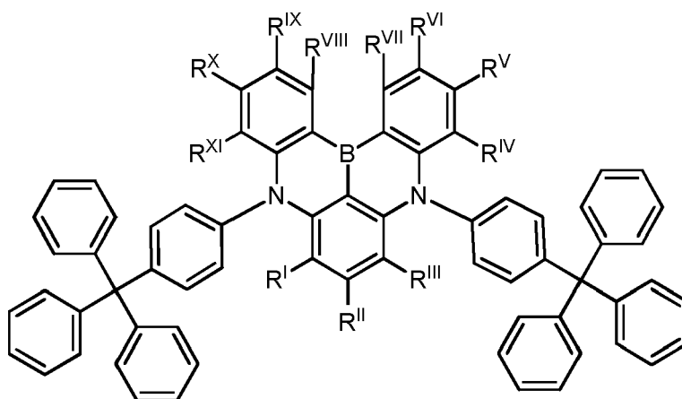
Formula III-1a
