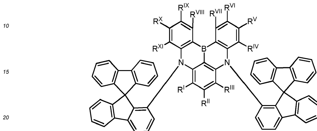
Formula V-1b
