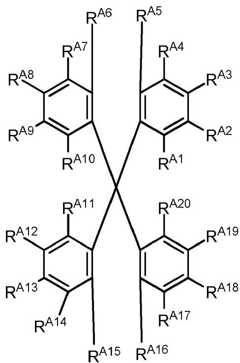
Formula IIe
