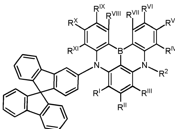
Formula IIIb
