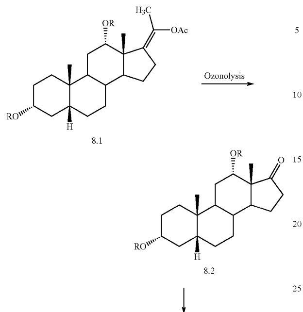
Scheme 8. Side-chain introduction
