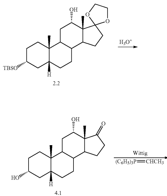
Scheme 4. Deprotection and Wittig Reaction
