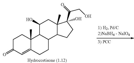
Scheme 1B. Synthesis of DCA from Hydrocortisone
