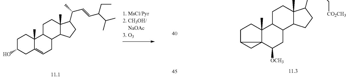
Scheme 11. Ozonolysis of i-steroid and side chain reduction
