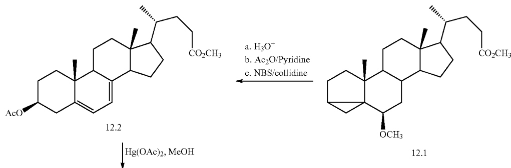
Scheme 12. Triene formation and allylic oxidation
