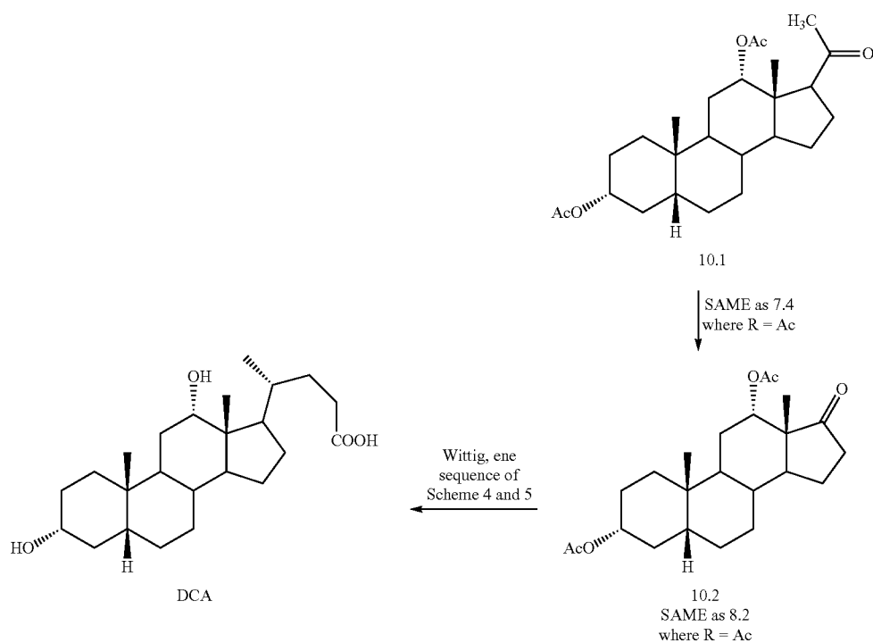
Scheme 10A. Formation DCA via the 3-keto-4-ene
