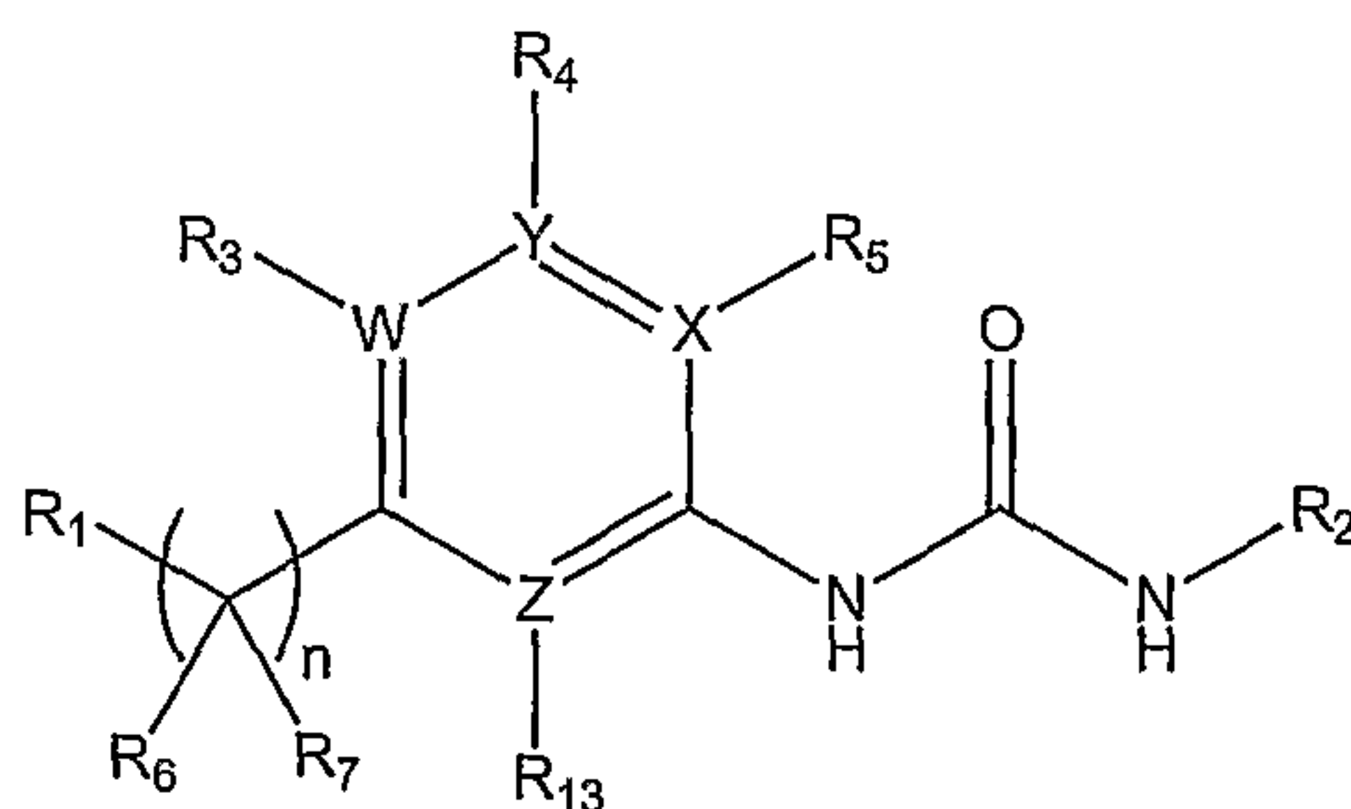
Formula I
