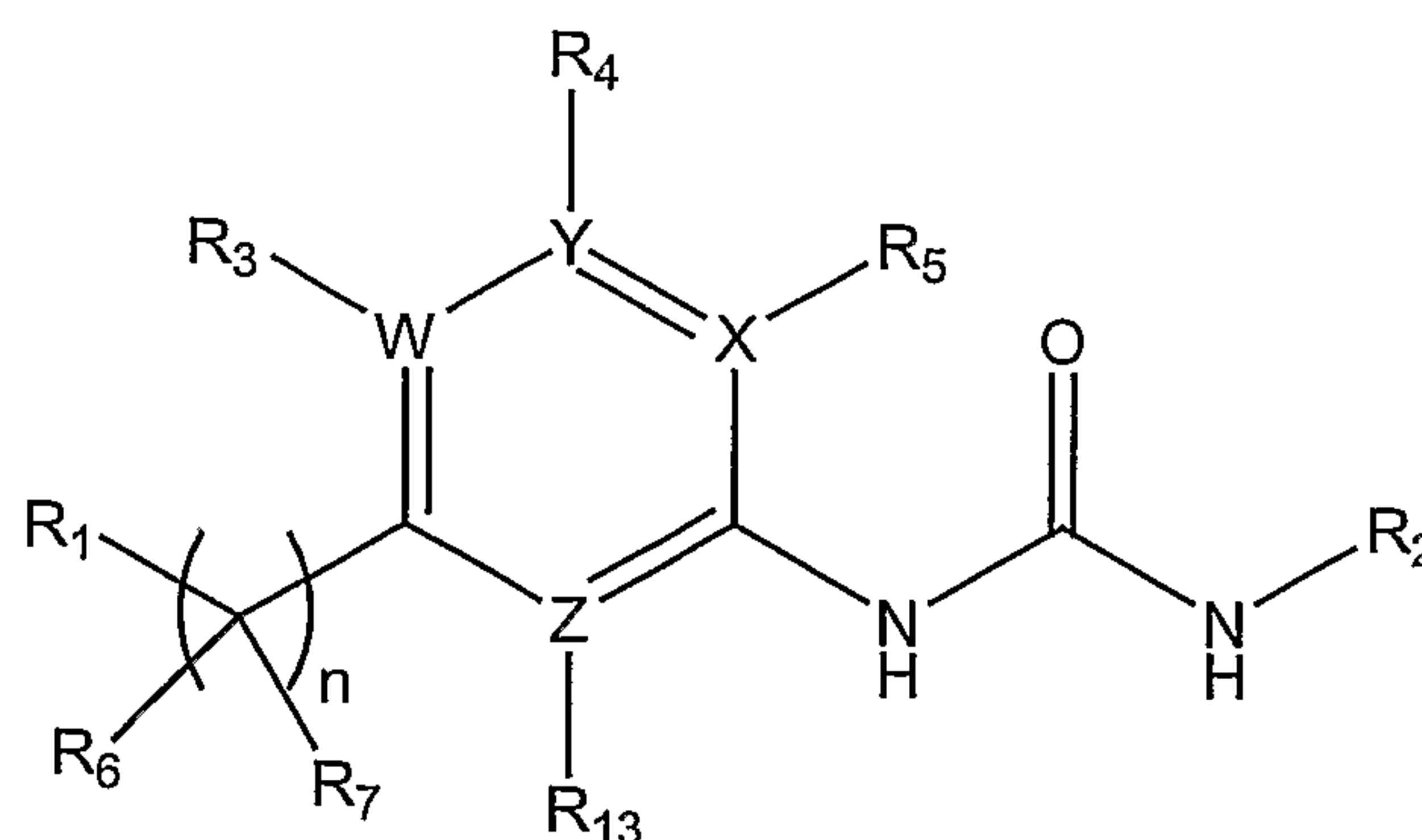
Formula I
