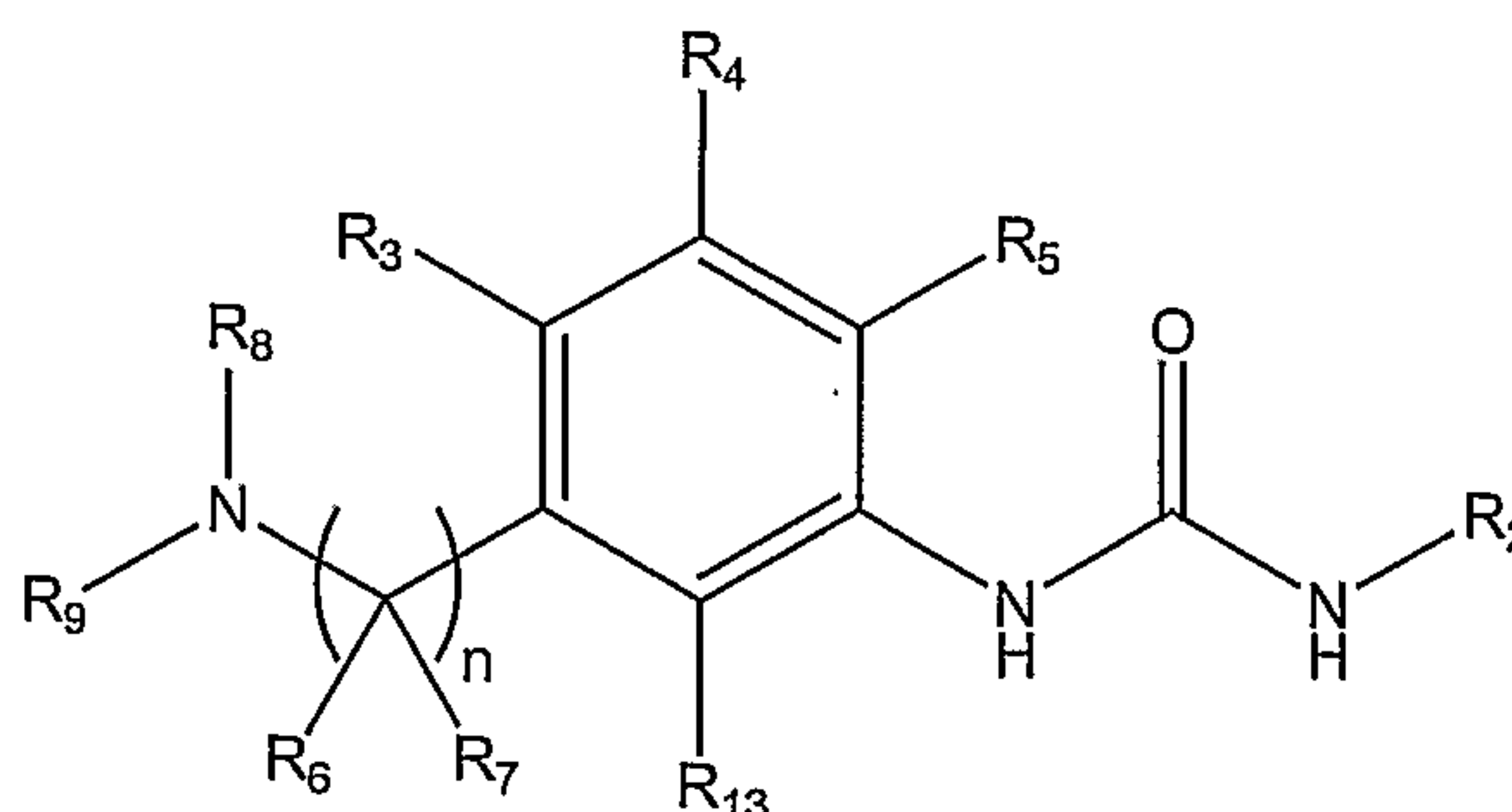
Formula Ib
