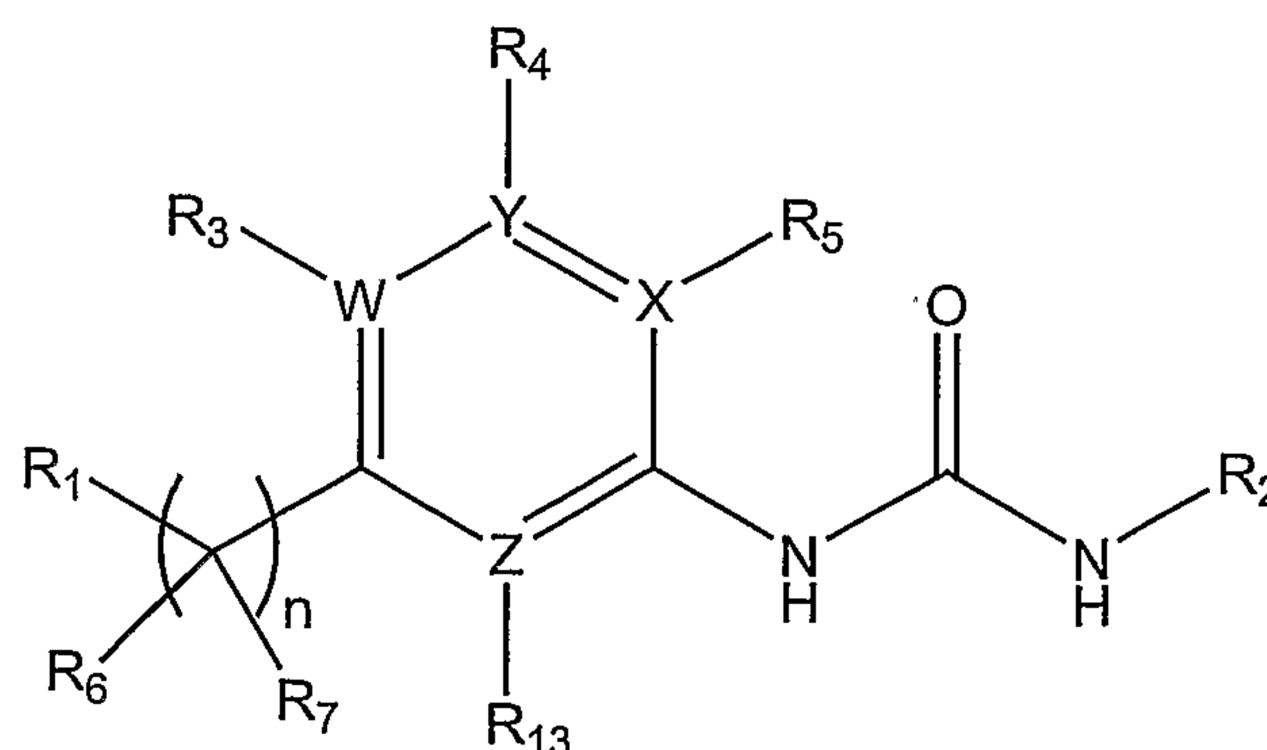
Formula I
