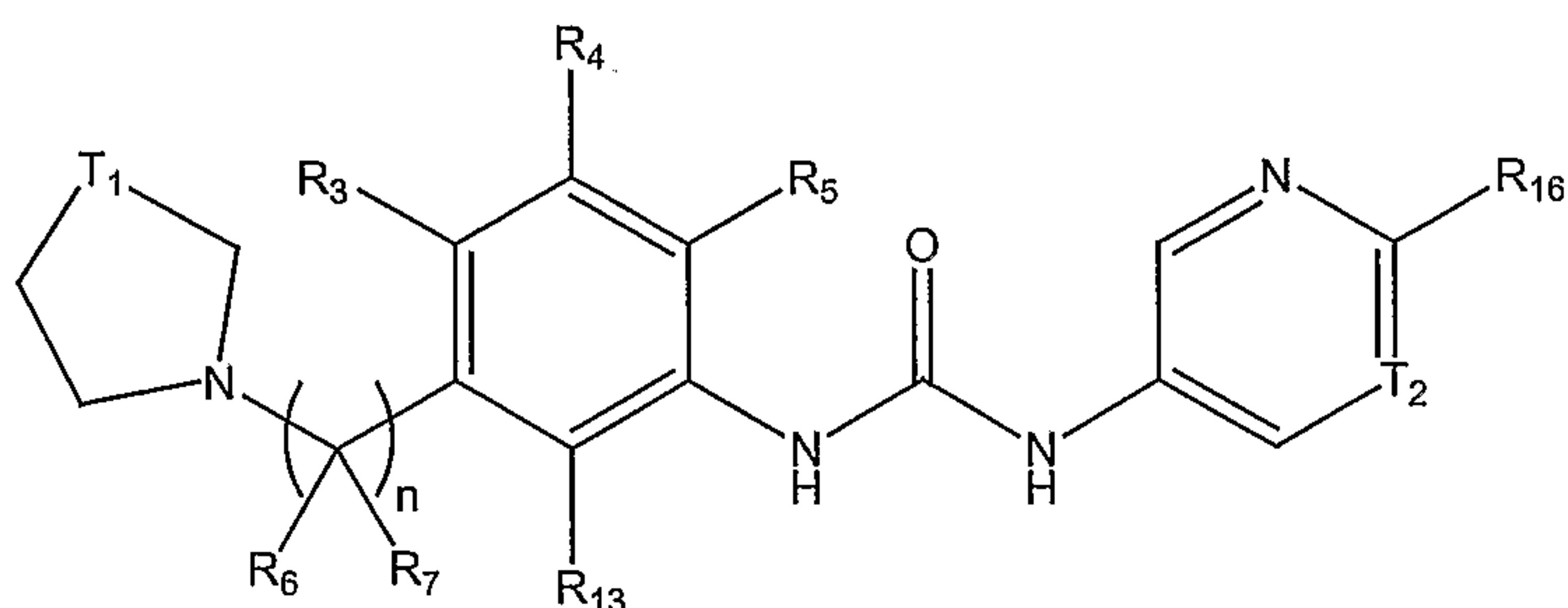
Formula Id
