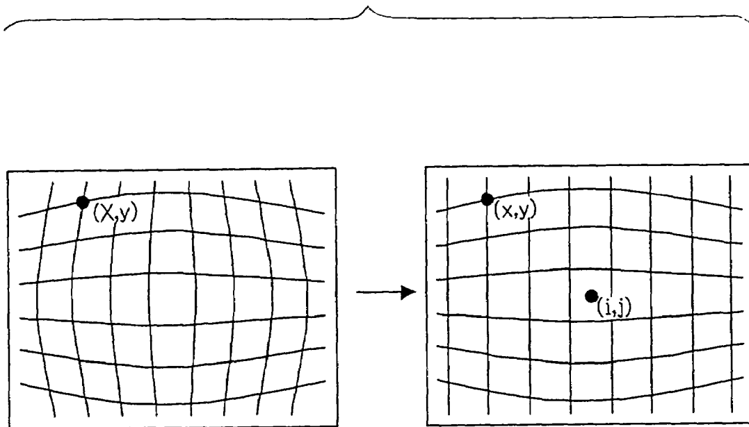
CORRECTION OF OPTICAL DISTORTION COMPONENT IN HORIZONTAL DIRECTION
