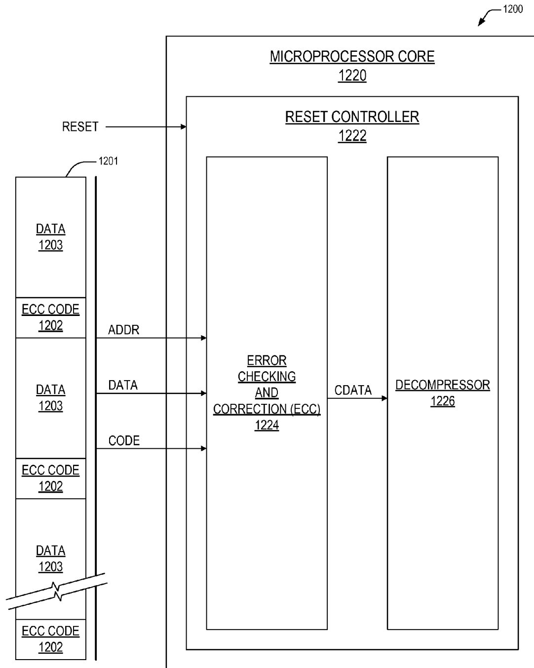
ERROR CHECKING AND CORRECTION (ECC) MECHNISM
