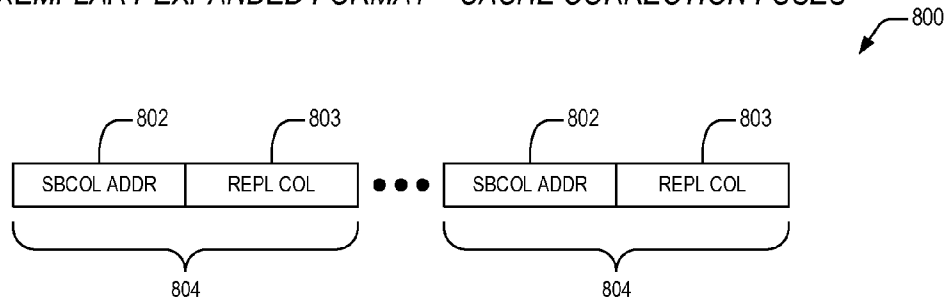
EXEMPLARY EXPANDED FORMAT – CACHE CORRECTION FUSES
