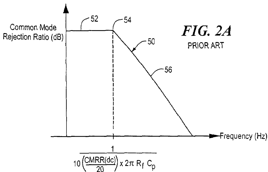
COMMON MODE REJECTION RATIO VS. FREQUENCY
