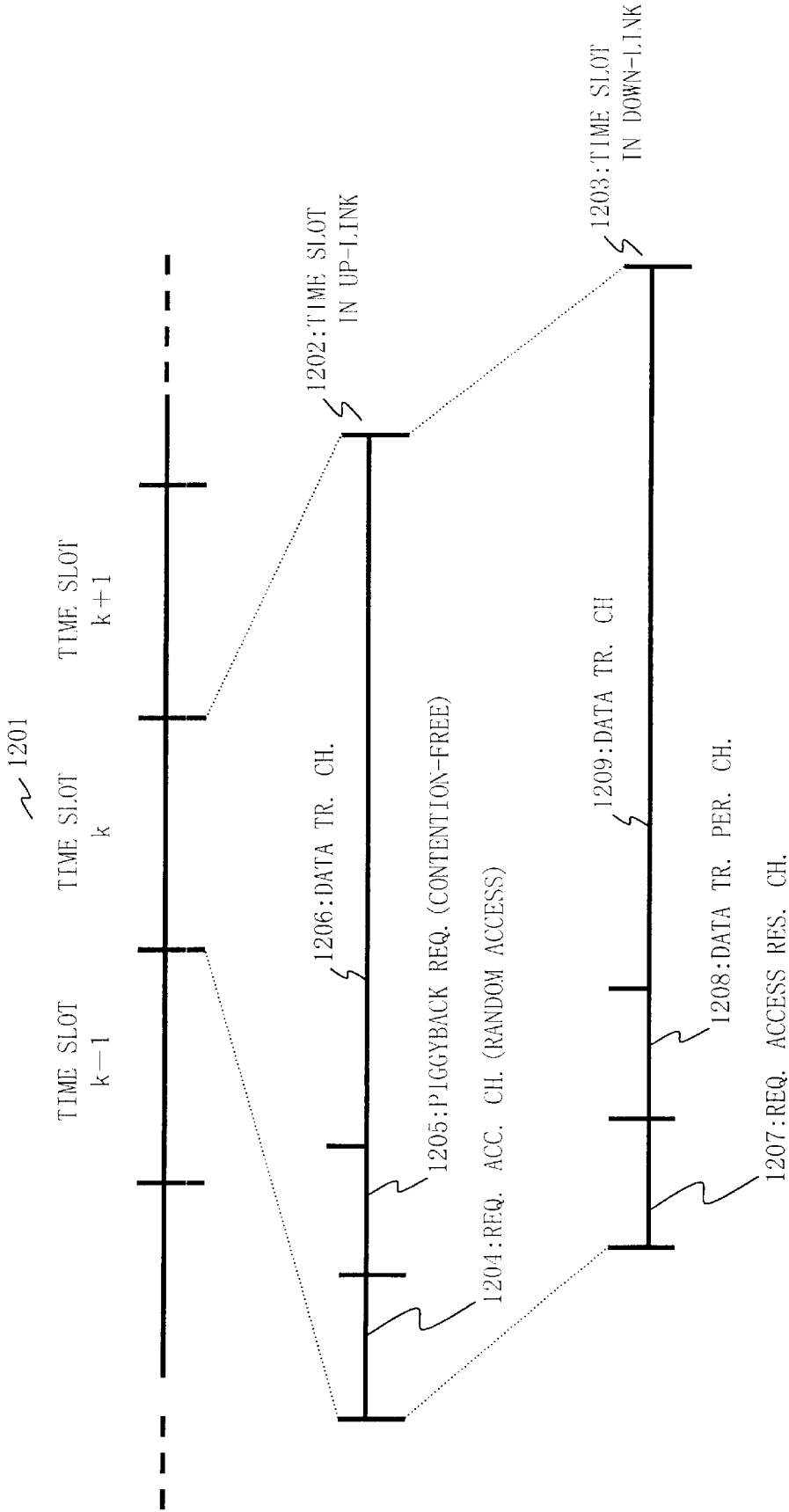
Fig. 12 RELATED ART
