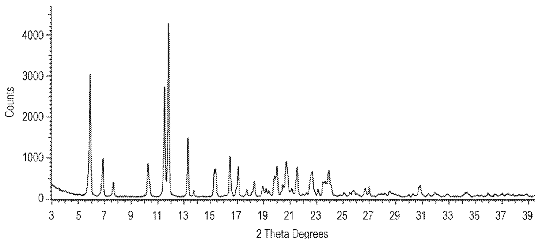
PXRD pattern of crystalline sodium salt of Example 5
