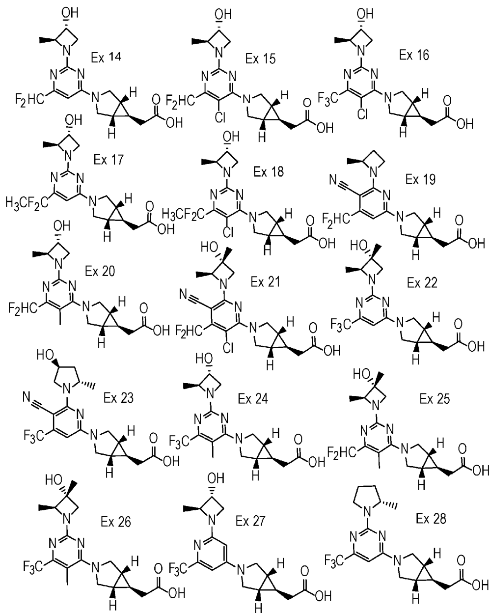
Structures of Examples in Table 4
