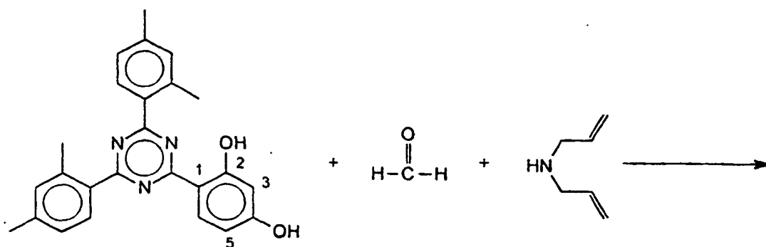
Compound A
