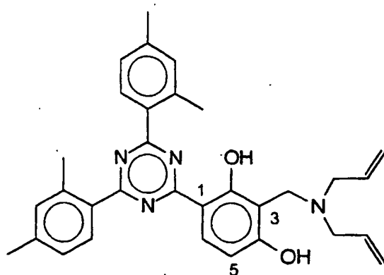
Compound B
