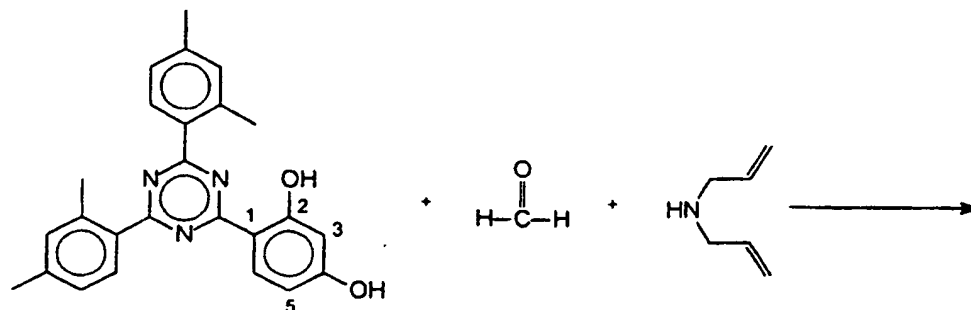
Compound A.
