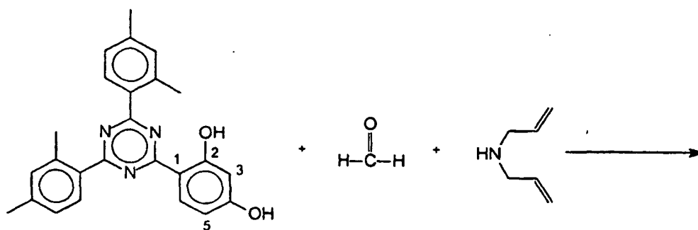
Compound A
