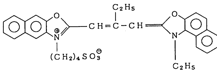
Sensitizing dye V
