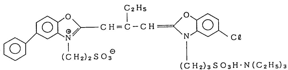
Sensitizing dye VI
