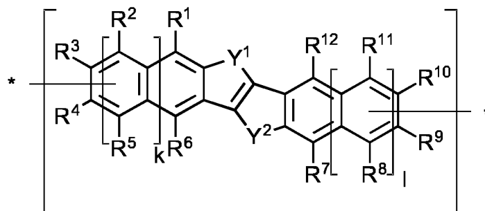
Formula (A)
