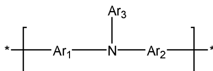
Formula (B)
