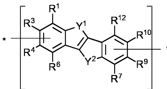
Formula (A2)
