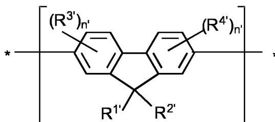
Formula (K)
