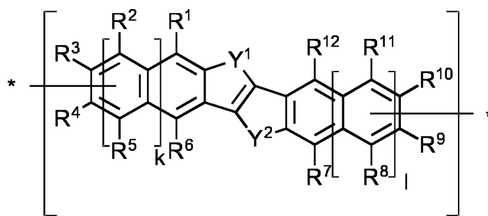
Formula (A)
