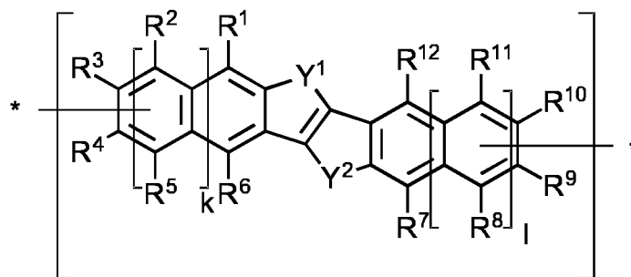
Formula (A1)
