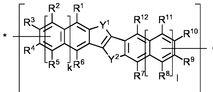
Formula (A1)
