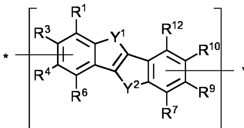
Formula (A2)
