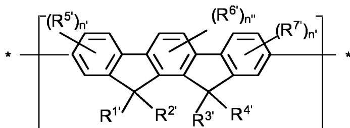
Formula (A)
