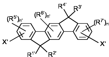
Structure (O/O')'
