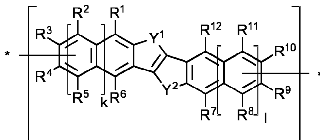
Formula (A)
