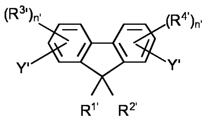
Structure K'
