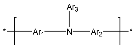
(P)
