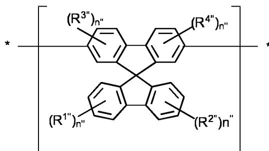
(R)
