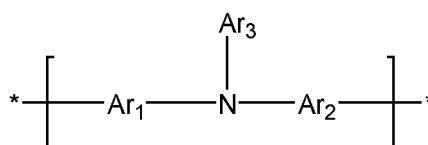
Formula (B)
