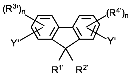
Structure K'
