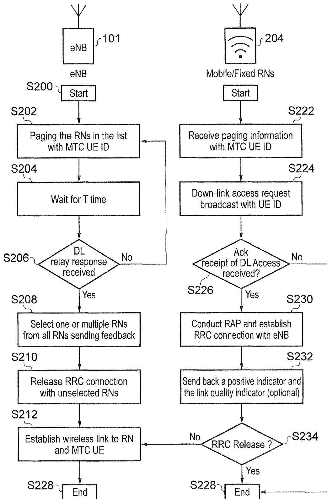
FIG. 11 Relay discovery for fixed RNs
