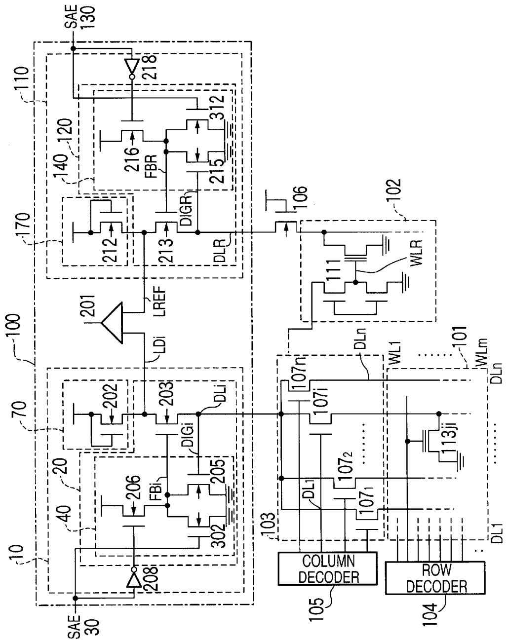
Fig. 2 PRIOR ART
