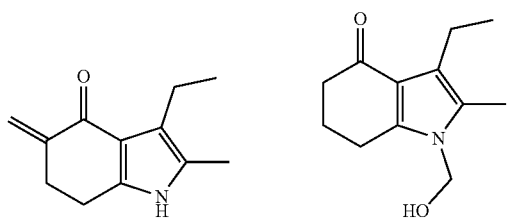
Methylene SUMO-2
