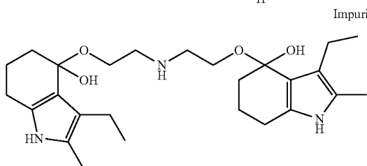
Impurity 3
