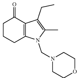
N-Morpholinomethyl SUMO-2
