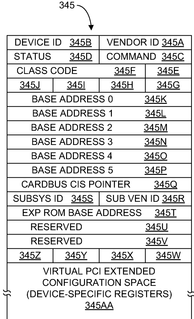
FIG. 2C (PRIOR ART)
