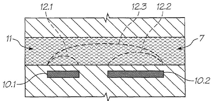
FIG. 52 (PRIOR ART)
