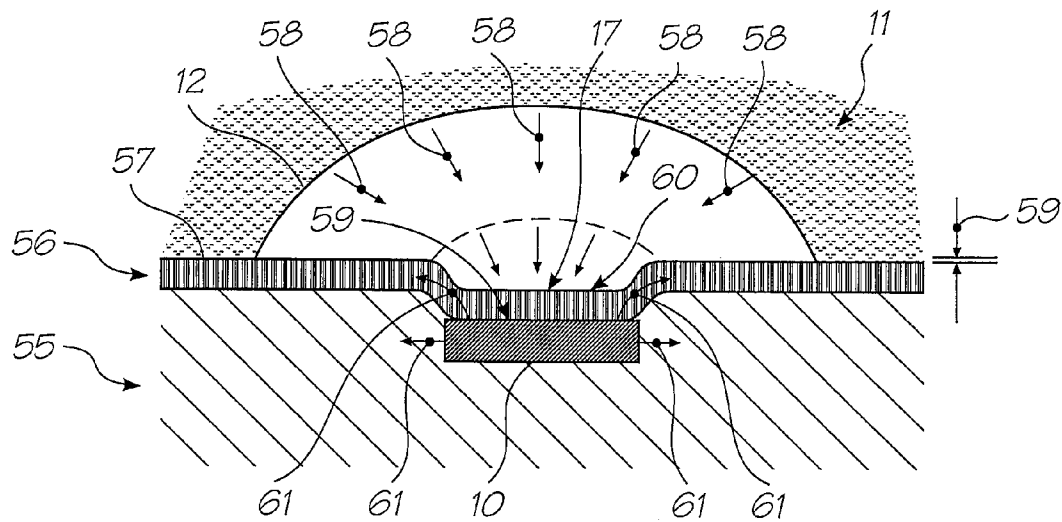
FIG. 47 (PRIOR ART)
