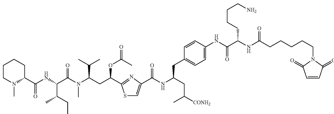
Amide of compound 39
