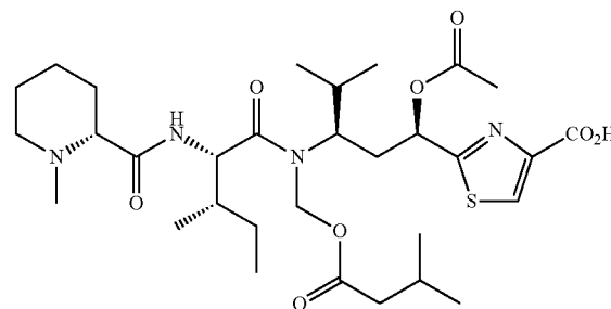
Acetate of Compound 27
