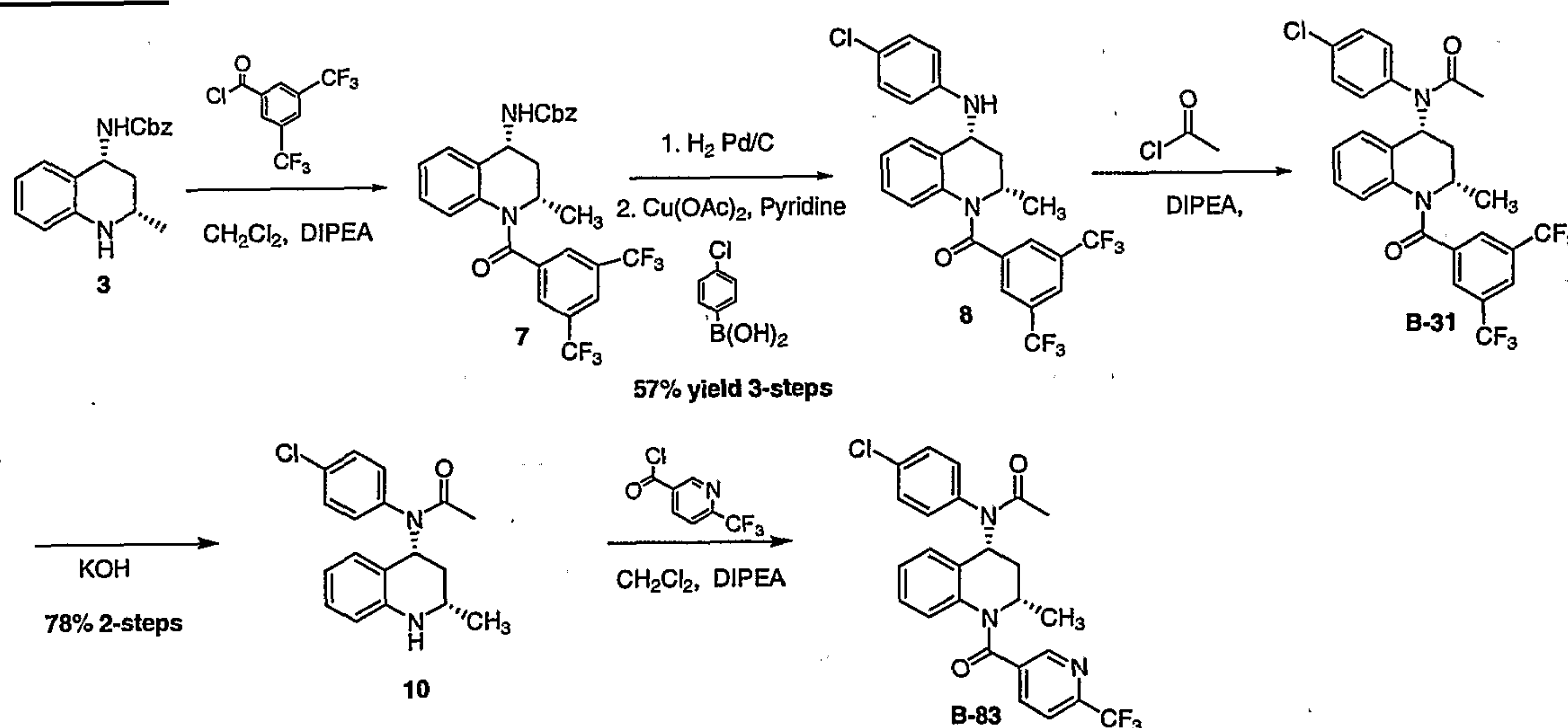
Scheme 22
