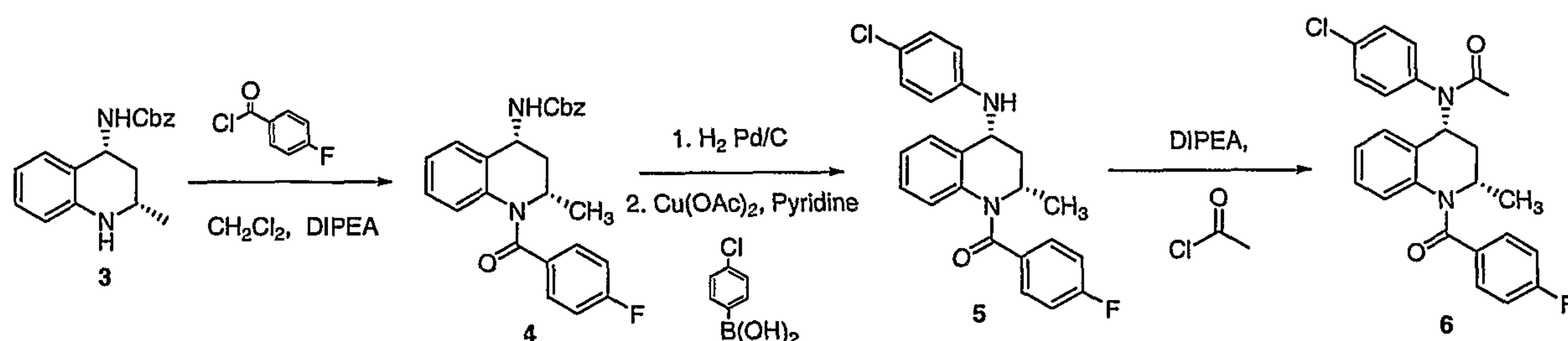
Scheme 21
