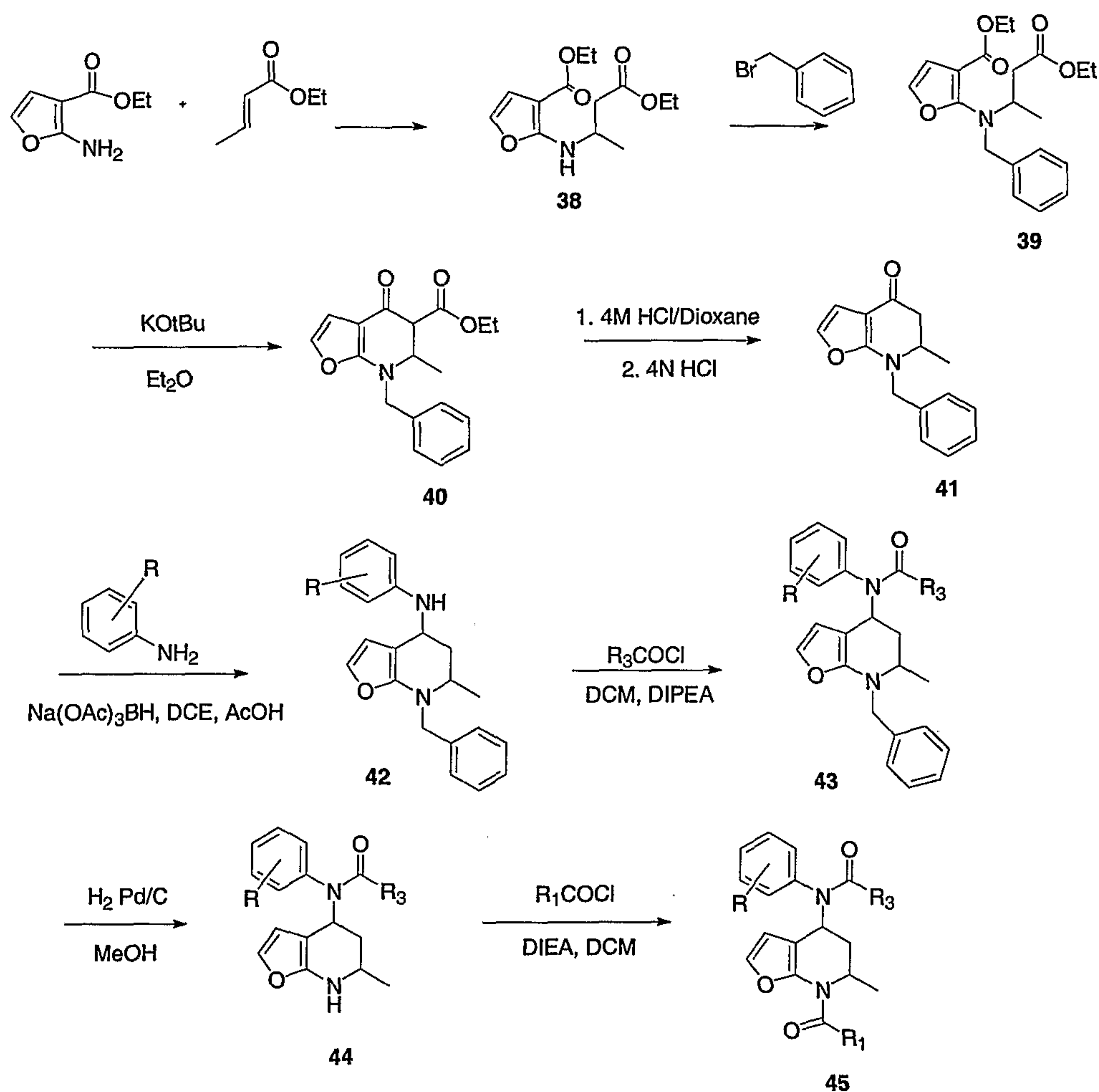
Scheme 16
