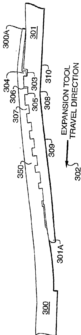
FIG. 3 (PRIOR ART)
