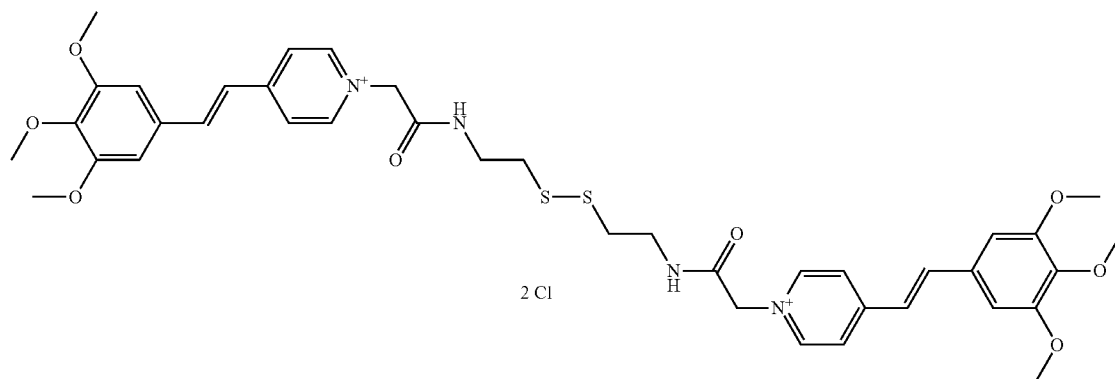
Synthesis scheme
