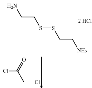
Synthesis scheme
