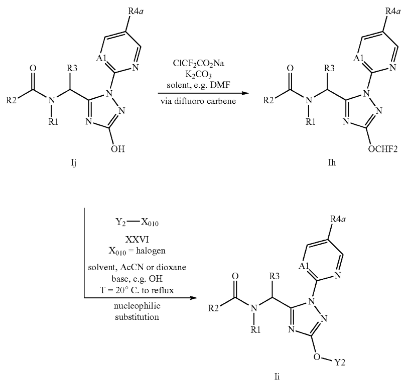
Scheme 11.
