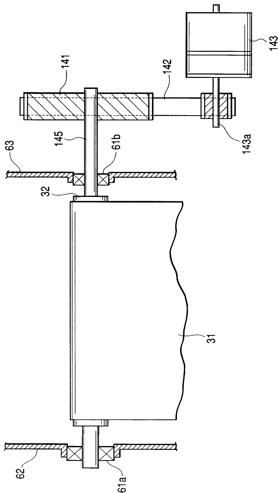
FIG. 5 PRIOR ART
