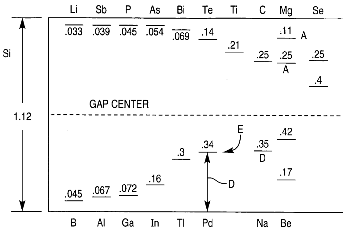
FIG. 8 PRIOR ART
