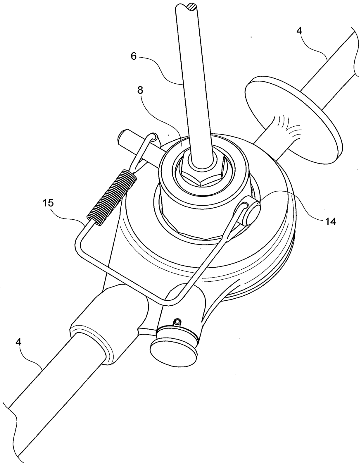
Fig.2 PRIOR ART
